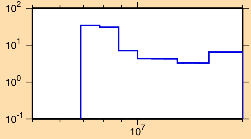
\Delta\sigma/\sigma vs. E for ^{47}\text{Ca}(n,2n)
