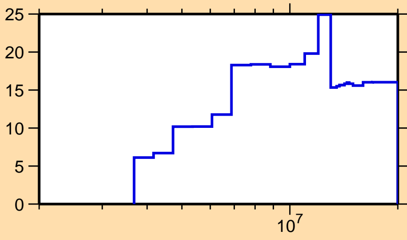
\Delta\sigma/\sigma vs. E for ^{47}\text{Ca}(n,n_1)
