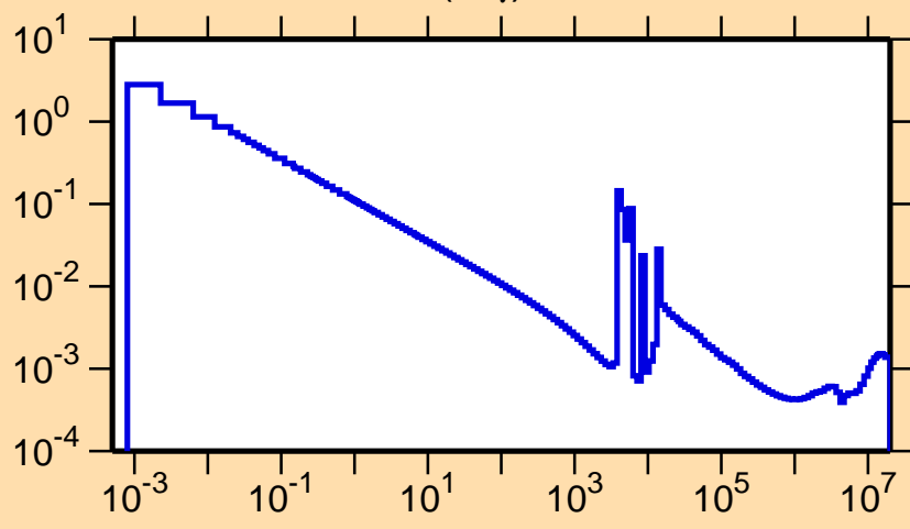
\sigma vs. E for ^{47}\text{Ca}(n,\gamma)
