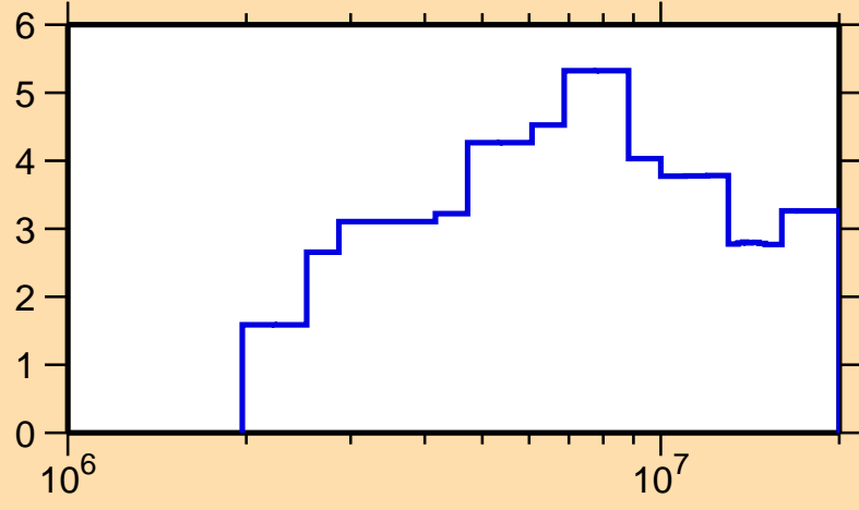
\Delta\sigma/\sigma vs. E for ^{47}\text{Ca}(n,\text{el.})
