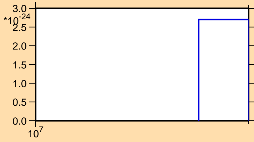
\sigma vs. E for ^{47}\text{Ca}(n,\text{He3})
