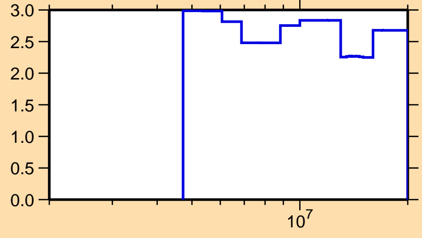
\Delta\sigma/\sigma vs. E for ^{47}\text{Ca}(n,n\text{onel.})
