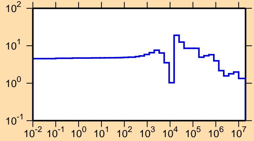
\Delta\sigma/\sigma vs. E for ^{47}\text{Ca}(n,\text{tot.})
