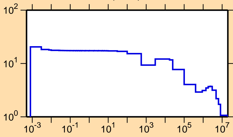
\sigma vs. E for ^{47}\text{Ca}(n,\text{el.})
