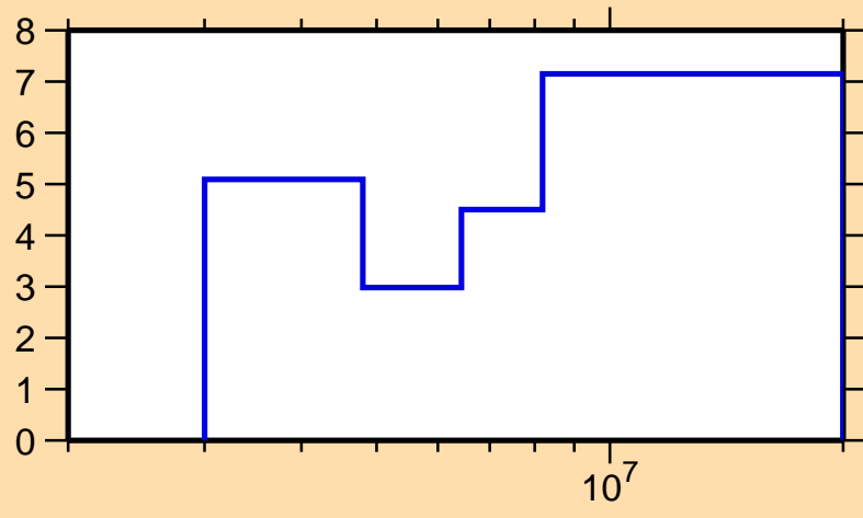
\Delta\sigma/\sigma vs. E for ^{47}\text{Ca}(n,\text{inel.})
