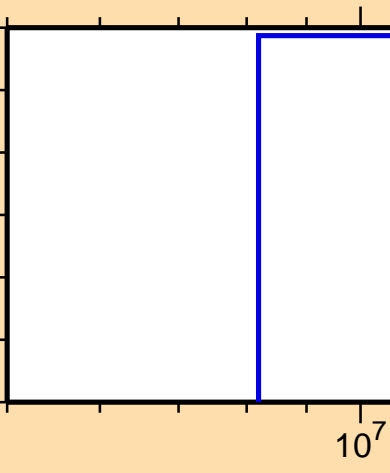
\sigma vs. E for ^{47}\text{Ca}(n,2n\alpha)
