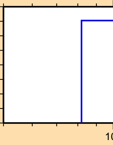
\sigma vs. E for ^{47}\text{Ca}(n,\text{nd})
