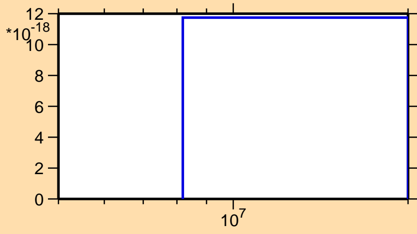
\sigma vs. E for ^{47}\text{Ca}(n,2n\alpha)
