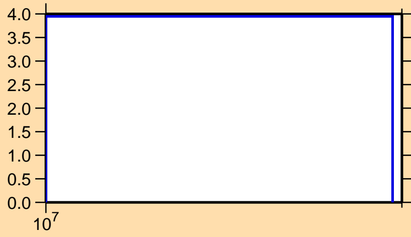
\Delta\sigma/\sigma vs. E for ^{48}\text{Ca}(n,ncont.)
