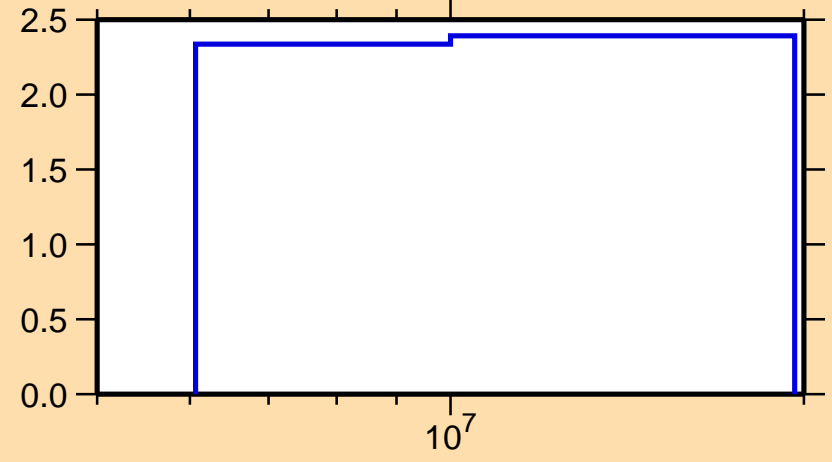
\Delta\sigma/\sigma vs. E for ^{48}\text{Ca}(n,\text{inel.})
