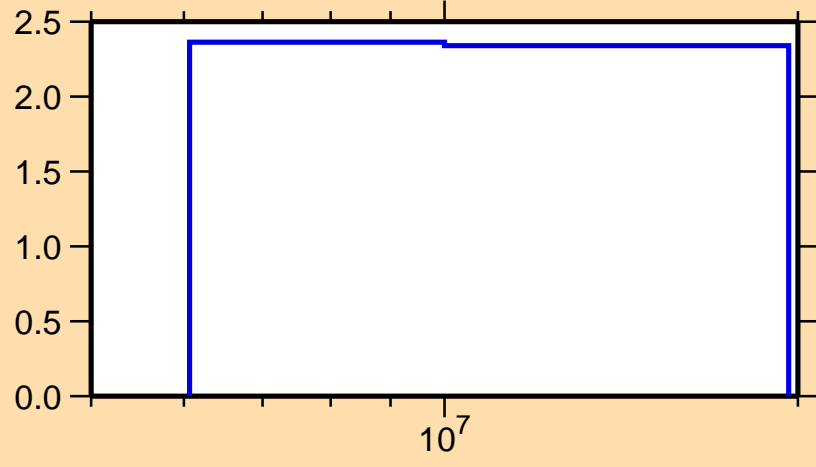
\Delta\sigma/\sigma vs. E for ^{48}\text{Ca}(n,n\text{nonel.})
