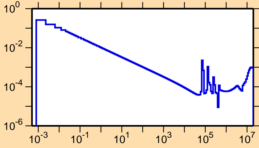
\sigma vs. E for ^{49}\text{Ca}(n,\gamma)
