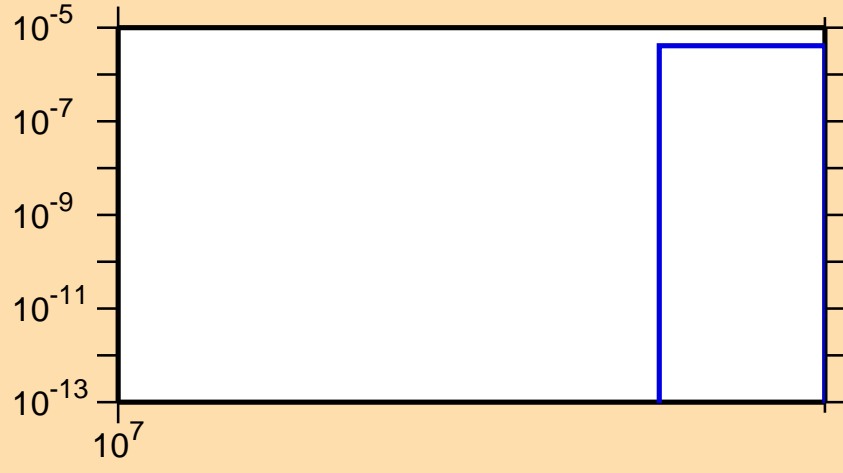
\sigma vs. E for ^{49}\text{Ca}(n,np)
