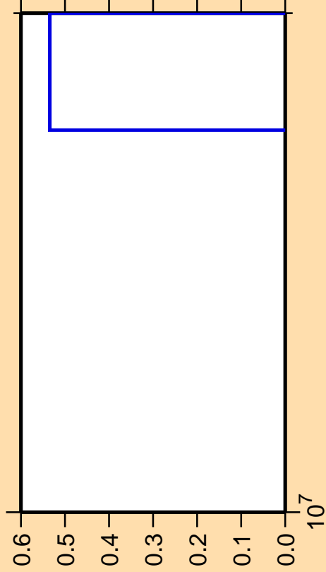
\Delta\sigma/\sigma vs. E for ^{49}\text{Ca}(n,\text{nd})
