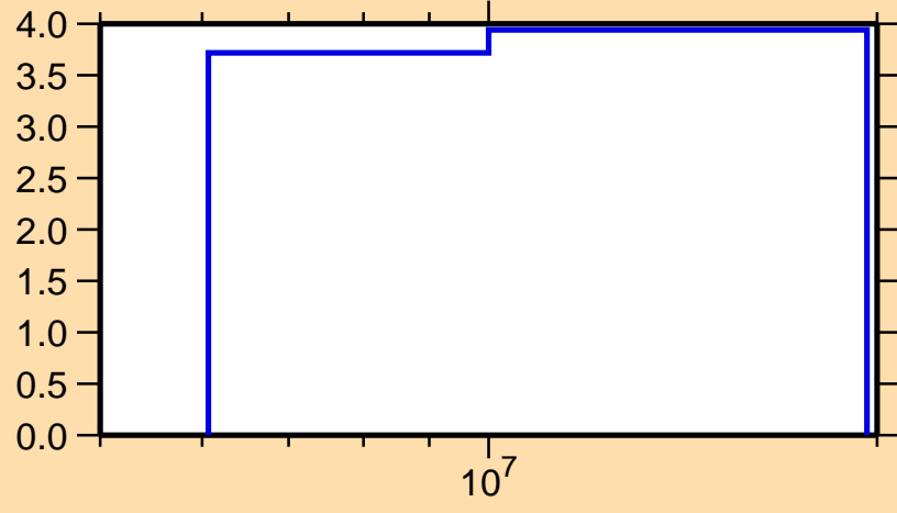
\Delta\sigma/\sigma vs. E for ^{49}\text{Ca}(n,n\text{nonel.})
