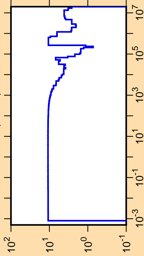
\Delta\sigma/\sigma vs. E for ^{50}\text{Ca}(n,\text{tot.})
