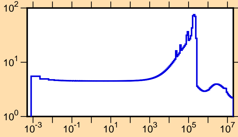
\sigma vs. E for ^{50}\text{Ca}(n,\text{tot.})
