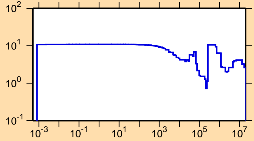
\Delta\sigma/\sigma vs. E for ^{50}\text{Ca}(n,\text{tot.})
