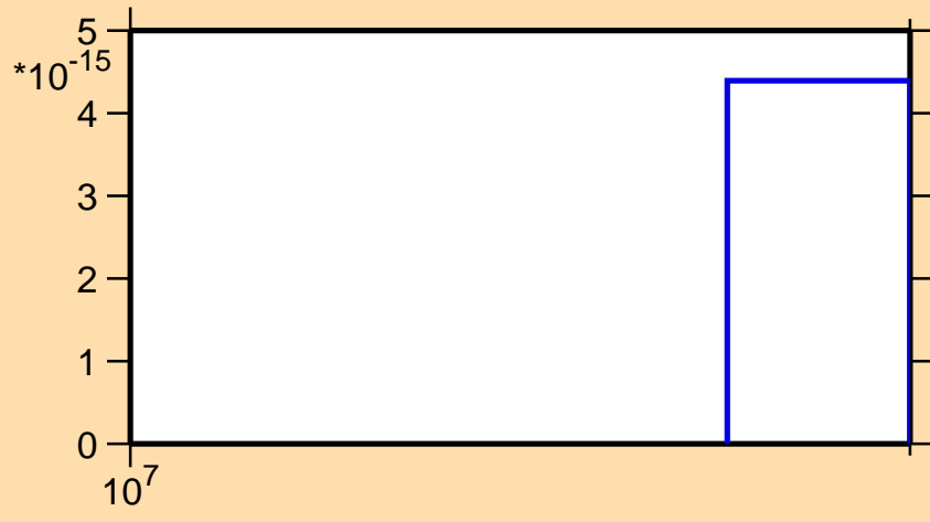
\sigma vs. E for ^{50}\text{Ca}(n,nt)
