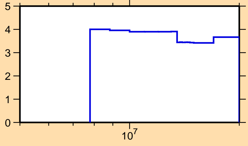
\Delta\sigma/\sigma vs. E for ^{50}\text{Ca}(n,n\text{onel.})
