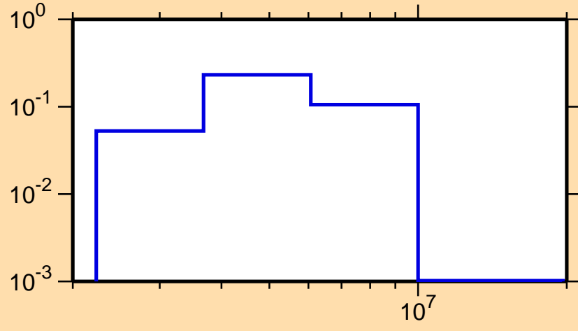
\sigma vs. E for ^{50}\text{Ca}(n,n_2)
