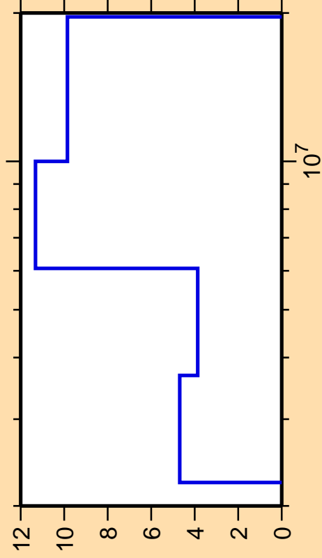
\Delta\sigma/\sigma vs. E for ^{50}\text{Ca}(n,n_2)
