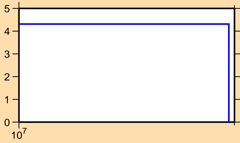
\Delta\sigma/\sigma vs. E for ^{50}\text{Ca}(n,2n)
