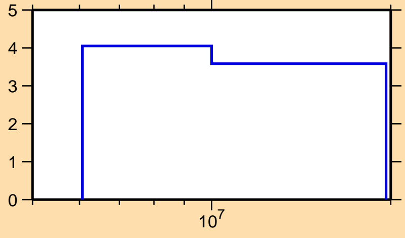
\Delta\sigma/\sigma vs. E for ^{50}\text{Ca}(n,n\text{nonel.})
