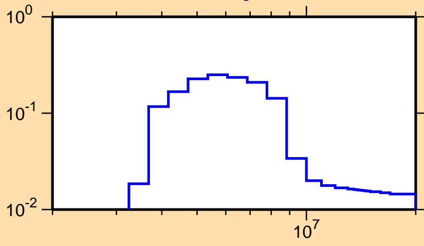
\sigma vs. E for ^{51}\text{Ca}(n,n_3)
