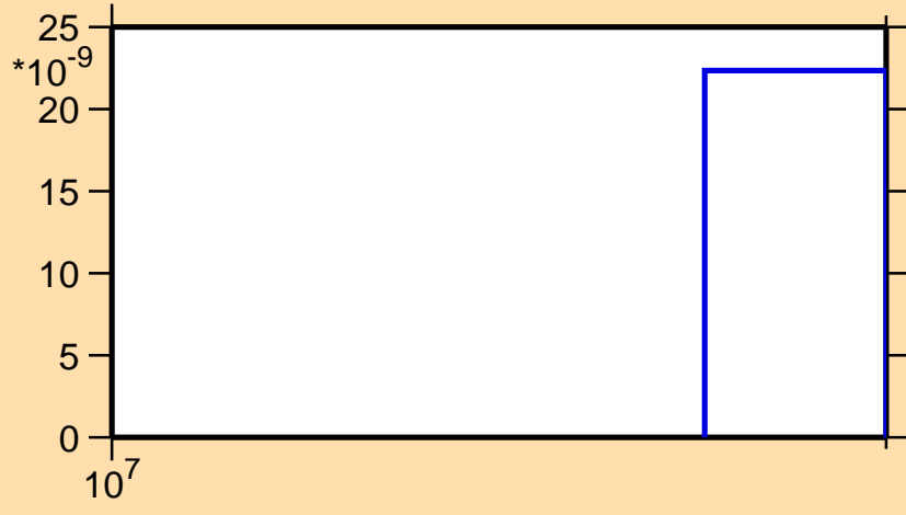
\sigma vs. E for ^{51}\text{Ca}(n,np)
