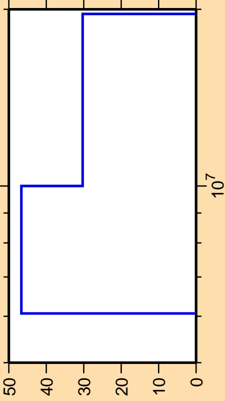
\Delta\sigma/\sigma vs. E for ^{51}\text{Ca}(n,n\text{cont.})
