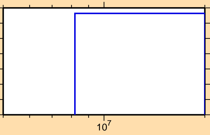
\sigma vs. E for ^{51}\text{Ca}(n,p)
