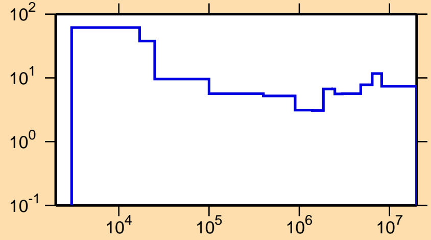
\Delta\sigma/\sigma vs. E for ^{51}\text{Ca}(n,\text{el.})
