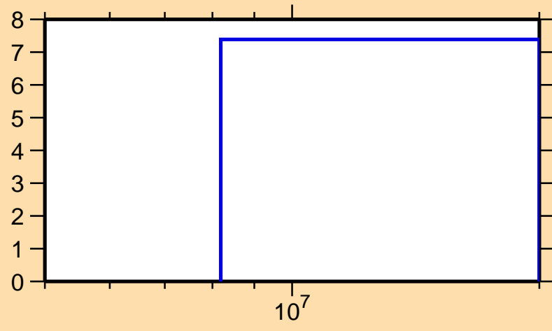
\Delta\sigma/\sigma vs. E for ^{51}\text{Ca}(n,el.)
