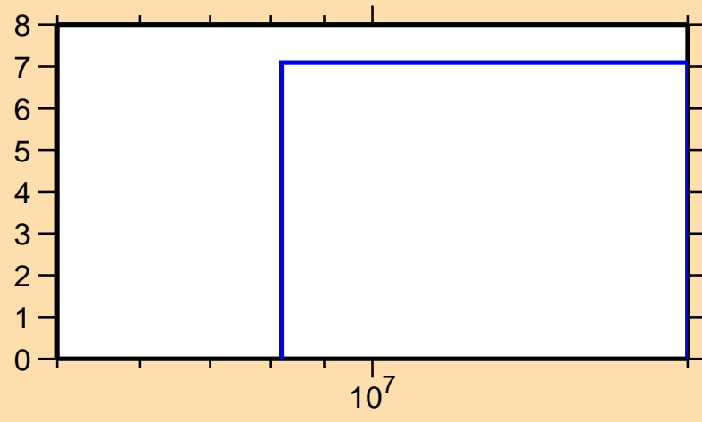
\Delta\sigma/\sigma vs. E for ^{51}\text{Ca}(n,2n)
