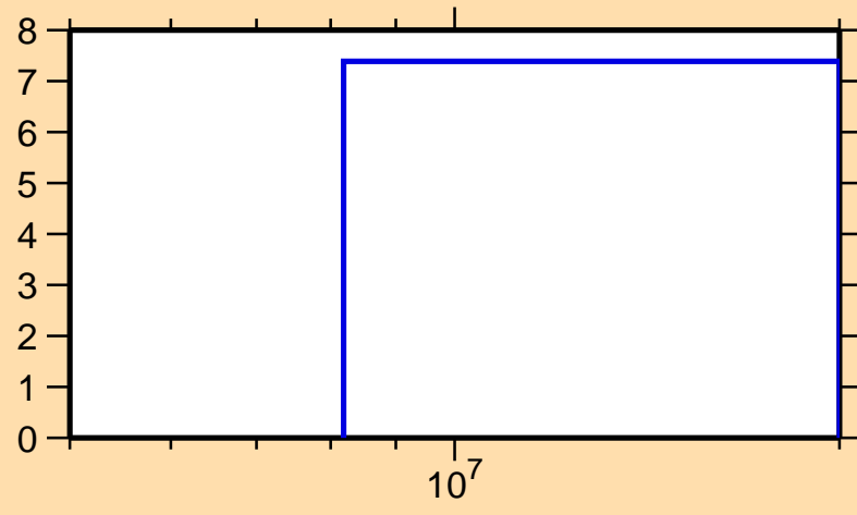
\Delta\sigma/\sigma vs. E for ^{51}\text{Ca}(n,\text{el.})
