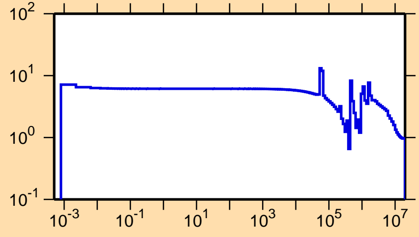
\sigma vs. E for ^{52}\text{Ca}(n,\text{el.})
