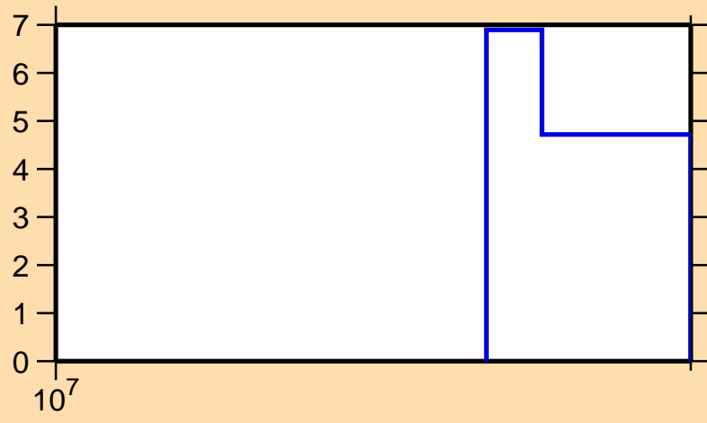
\Delta\sigma/\sigma vs. E for ^{52}\text{Ca}(n,el.)
