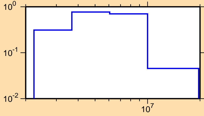
\sigma vs. E for ^{52}\text{Ca}(n,n_1)
