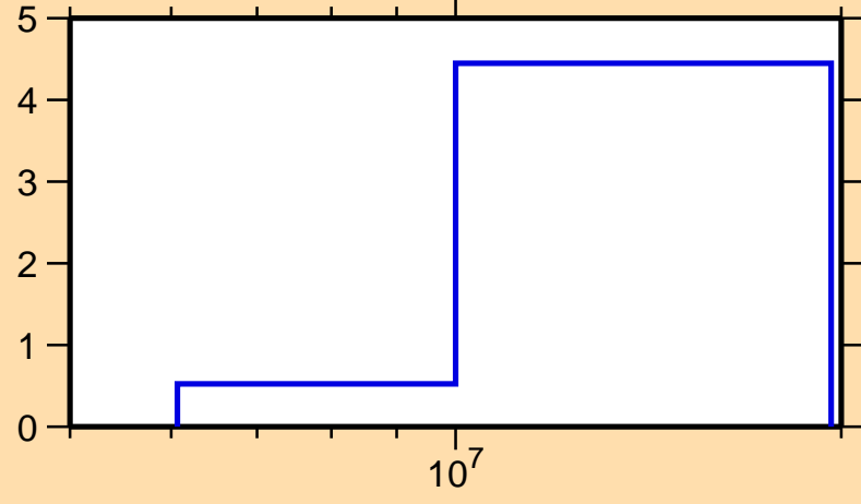
\Delta\sigma/\sigma vs. E for ^{52}\text{Ca}(n,2n)
