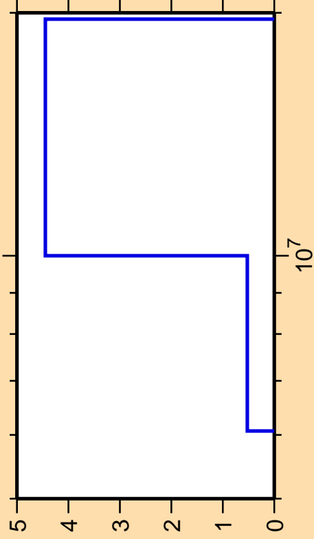
\Delta\sigma/\sigma vs. E for ^{52}\text{Ca}(n,2n)
