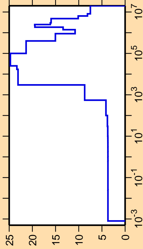
\Delta\sigma/\sigma vs. E for ^{97}\text{Cd}(n,\text{el.})
