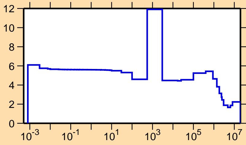
\sigma vs. E for ^{97}\text{Cd}(n,\text{el.})
