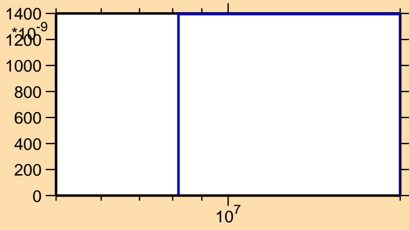
\sigma vs. E for ^{97}\text{Cd}(n,n\alpha)
