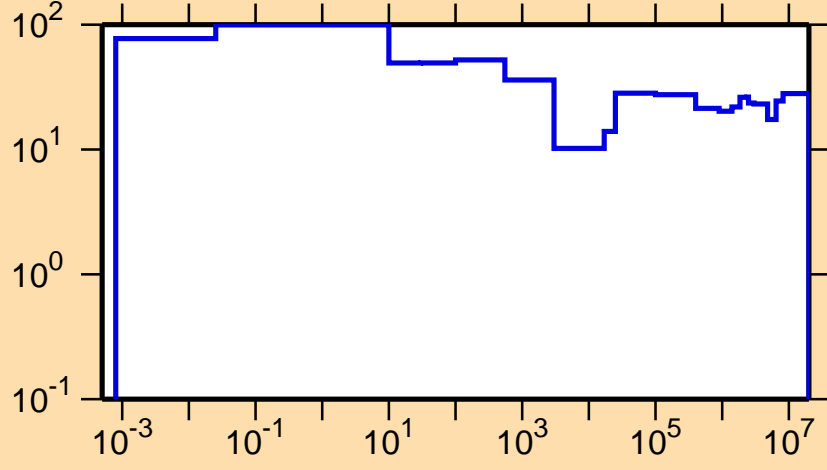
\Delta\sigma/\sigma vs. E for ^{97}\text{Cd}(n,p)
