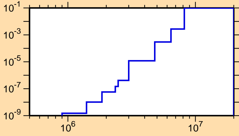
\sigma vs. E for ^{97}\text{Cd}(n,p\alpha)
