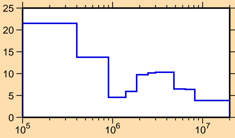
\Delta\sigma/\sigma vs. E for ^{97}\text{Cd}(n, tot.)
