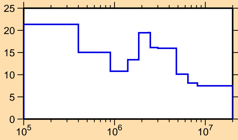
\Delta\sigma/\sigma vs. E for ^{97}\text{Cd}(n, el.)
