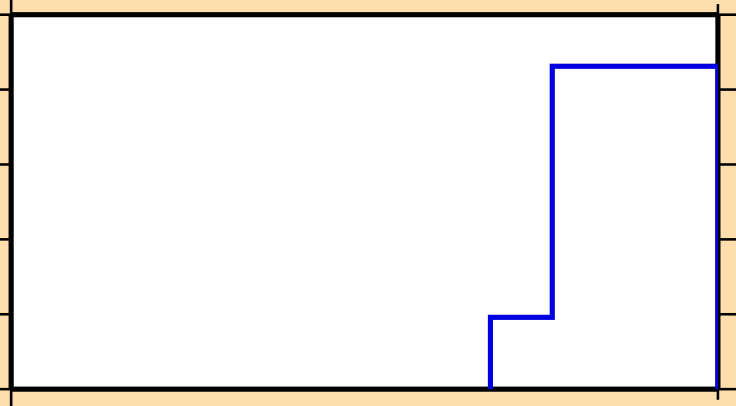
\sigma vs. E for ^{98}\text{Cd}(n,\text{pt})
