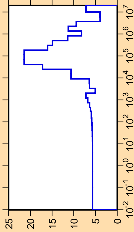
\Delta\sigma/\sigma vs. E for ^{98}\text{Cd}(n,\text{el.})
