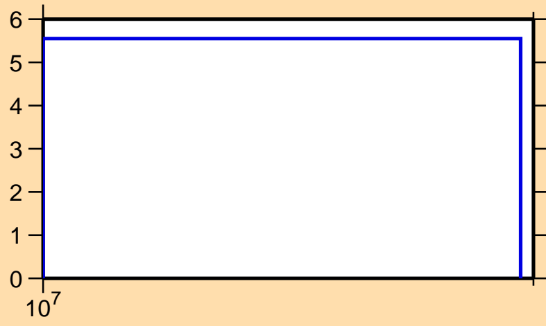
\Delta\sigma/\sigma vs. E for ^{98}\text{Cd}(n,\text{nonel.})
