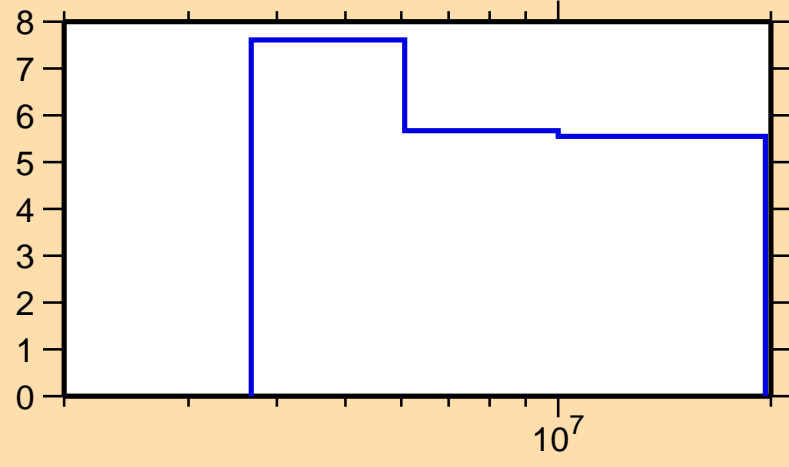
\Delta\sigma/\sigma vs. E for ^{98}\text{Cd}(n,n\text{nonel.})
