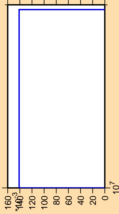
\Delta\sigma/\sigma vs. E for ^{98}\text{Cd}(n,\text{nd})
