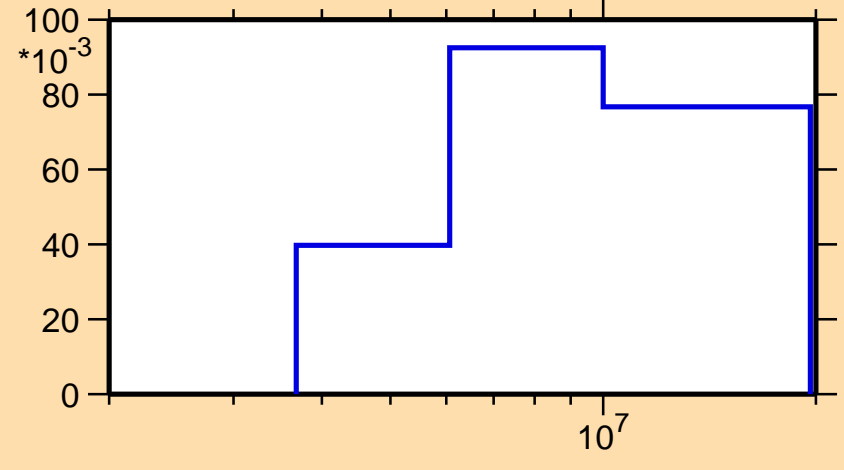
\sigma vs. E for ^{98}\text{Cd}(n,n\text{cont.})
