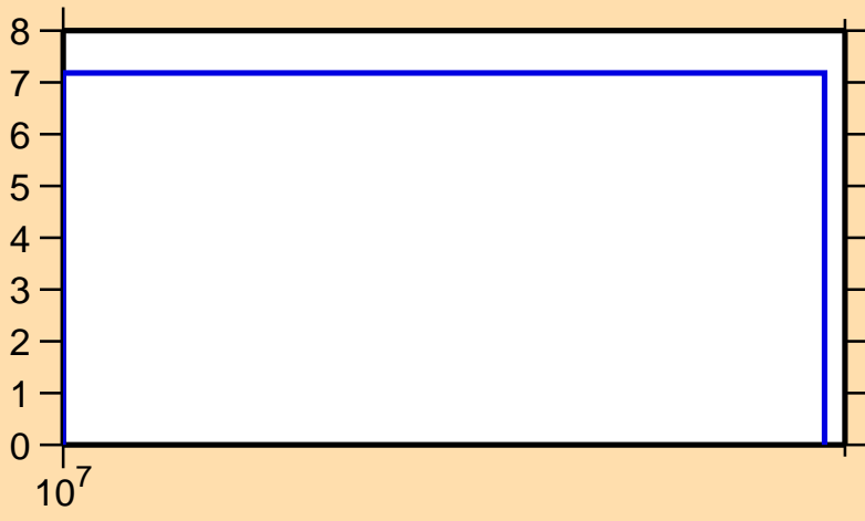
\Delta\sigma/\sigma vs. E for ^{98}\text{Cd}(n,\text{el.})
