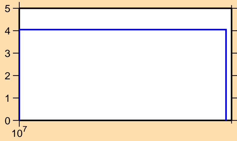
\Delta\sigma/\sigma vs. E for ^{98}\text{Cd}(n,\text{tot.})
