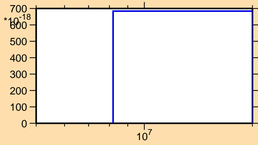
\sigma vs. E for ^{98}\text{Cd}(n,2np)
