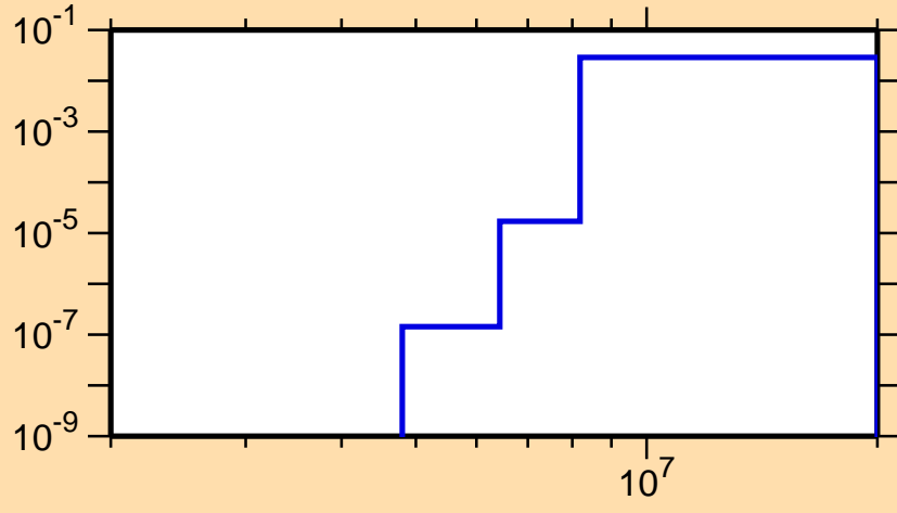
\sigma vs. E for ^{98}\text{Cd}(n,p\alpha)
