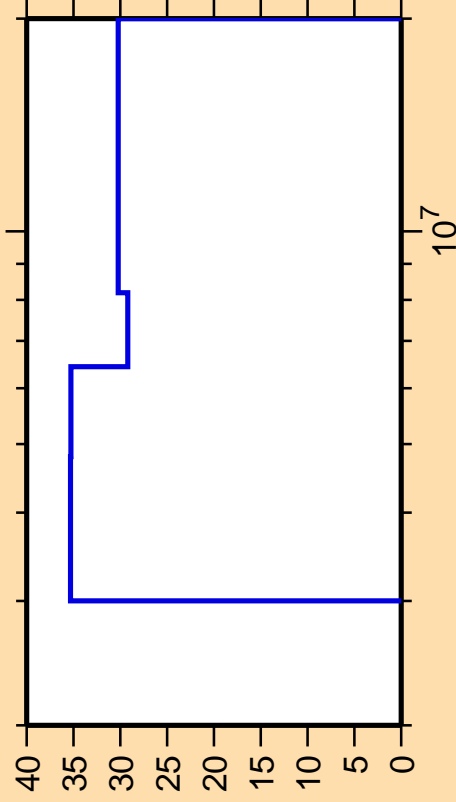
\Delta\sigma/\sigma vs. E for ^{98}\text{Cd}(n,\text{ncont.})
