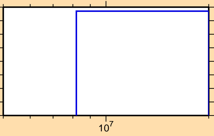
\sigma vs. E for ^{98}\text{Cd}(n,n\alpha)
