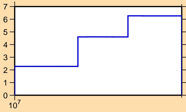
\Delta\sigma/\sigma vs. E for ^{99}\text{Cd}(n,\text{tot.})
