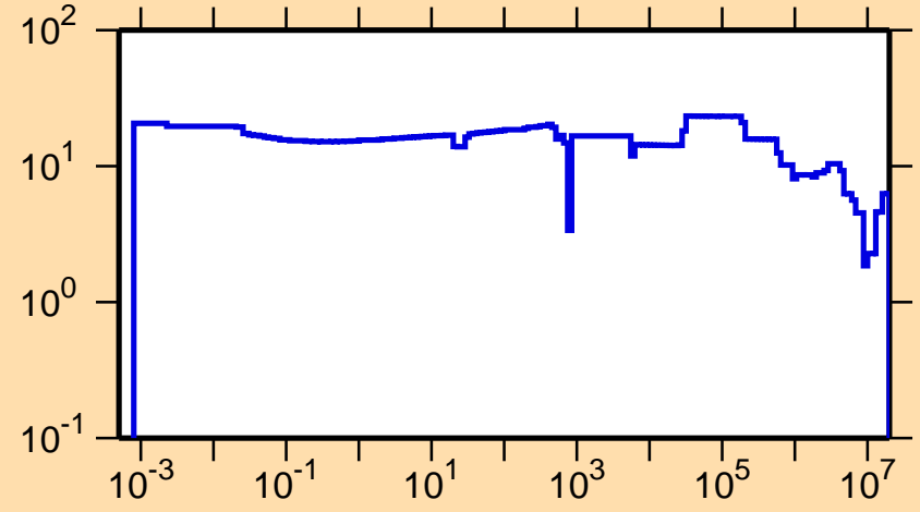
\Delta\sigma/\sigma vs. E for ^{99}\text{Cd}(n,\text{tot.})
