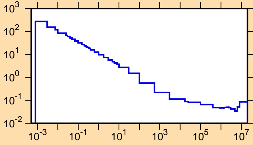
\sigma vs. E for ^{99}\text{Cd}(n,\alpha)
