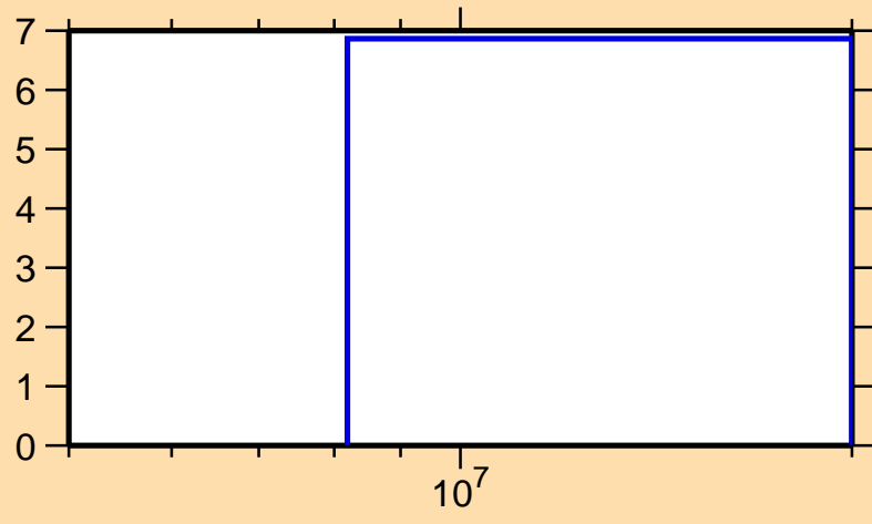
\Delta\sigma/\sigma vs. E for ^{99}\text{Cd}(n,\text{el.})
