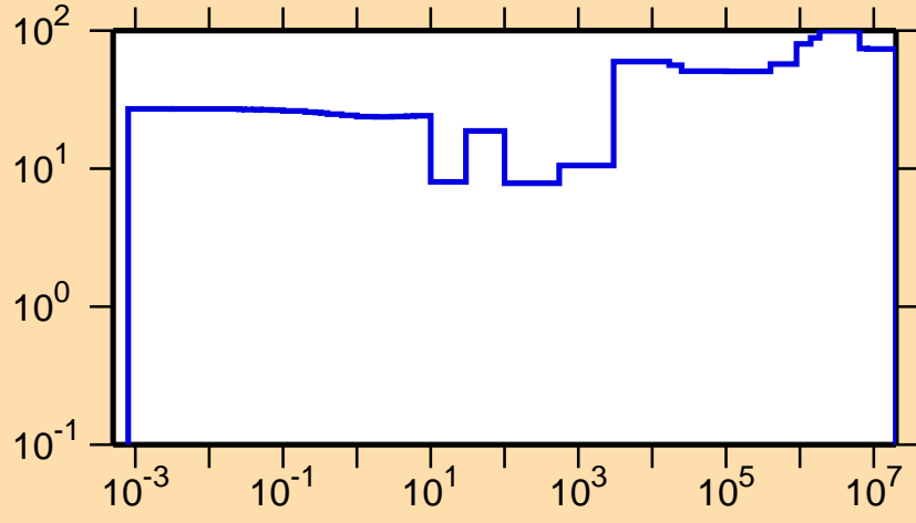
\Delta\sigma/\sigma vs. E for ^{99}\text{Cd}(n,\gamma)
