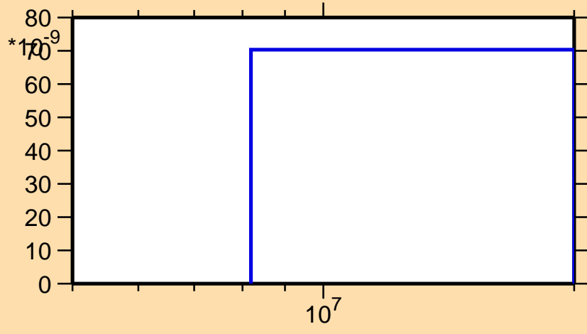
\sigma vs. E for ^{99}\text{Cd}(n,\text{nd})
