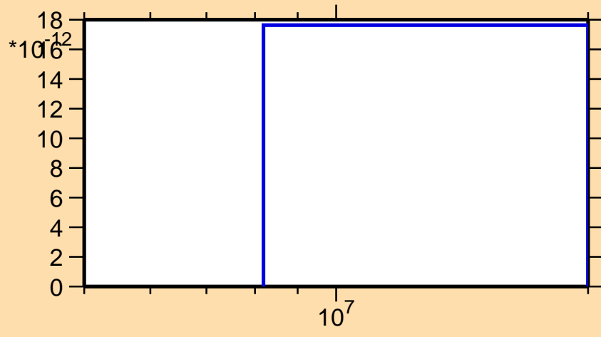
\sigma vs. E for ^{99}\text{Cd}(\text{mt117})
