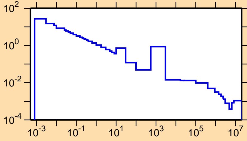
\sigma vs. E for ^{99}\text{Cd}(n,\gamma)
