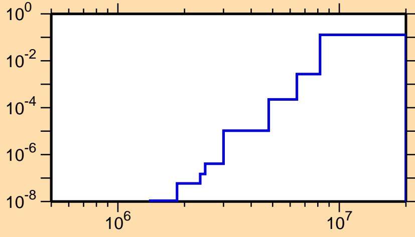
\sigma vs. E for ^{99}\text{Cd}(n,p\alpha)
