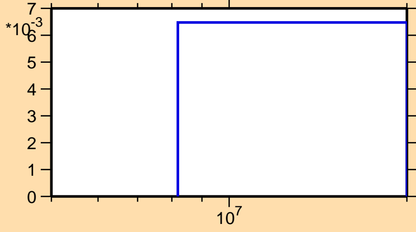
\sigma vs. E for ^{99}\text{Cd}(n,2n)
