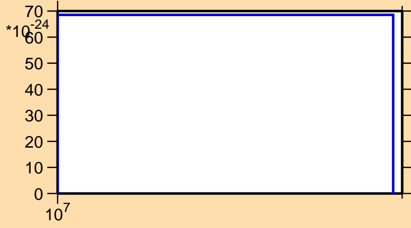
\sigma vs. E for ^{100}\text{Cd}(n,nt)
