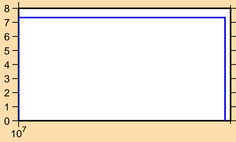
\Delta\sigma/\sigma vs. E for ^{100}\text{Cd}(n,\text{el.})
