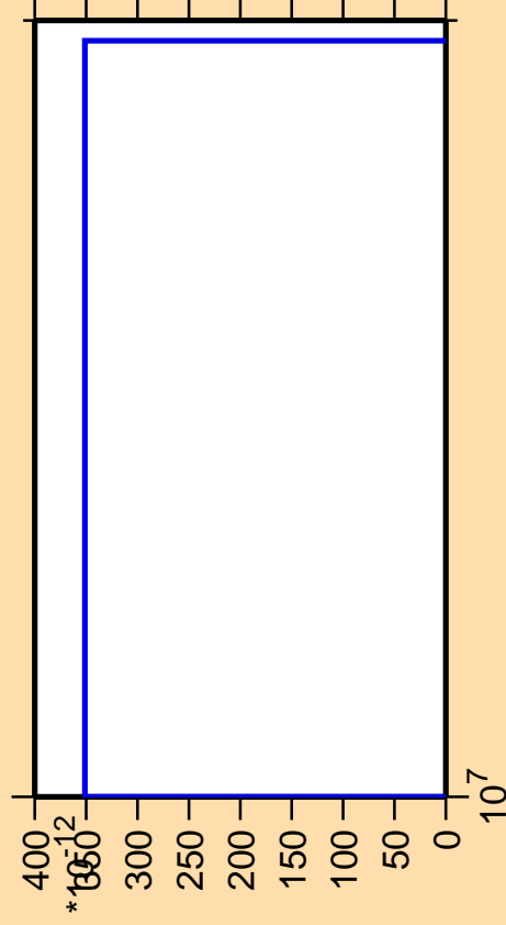
\Delta\sigma/\sigma vs. E for ^{100}\text{Cd}(n,nt)
