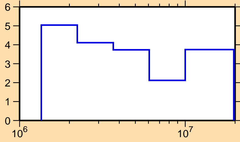
\Delta\sigma/\sigma vs. E for ^{100}\text{Cd}(n,\text{tot.})
