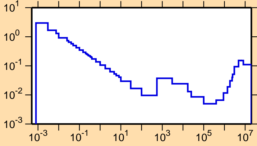
\sigma vs. E for ^{100}\text{Cd}(n,\alpha)
