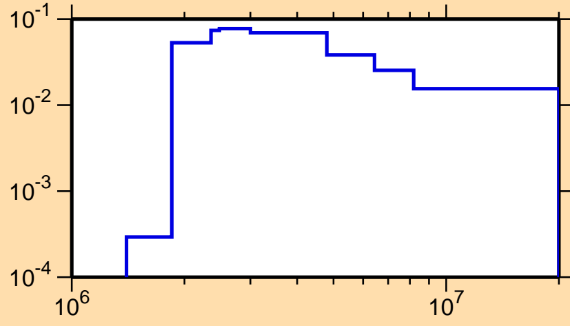
\sigma vs. E for ^{100}\text{Cd}(n,n_2)
