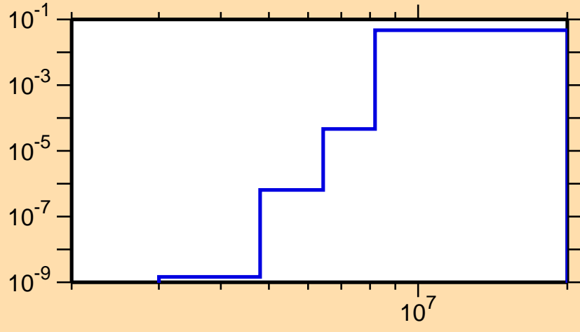
\sigma vs. E for ^{100}\text{Cd}(n,p\alpha)
