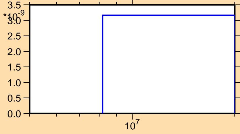
\sigma vs. E for ^{100}\text{Cd}(n,2np)
