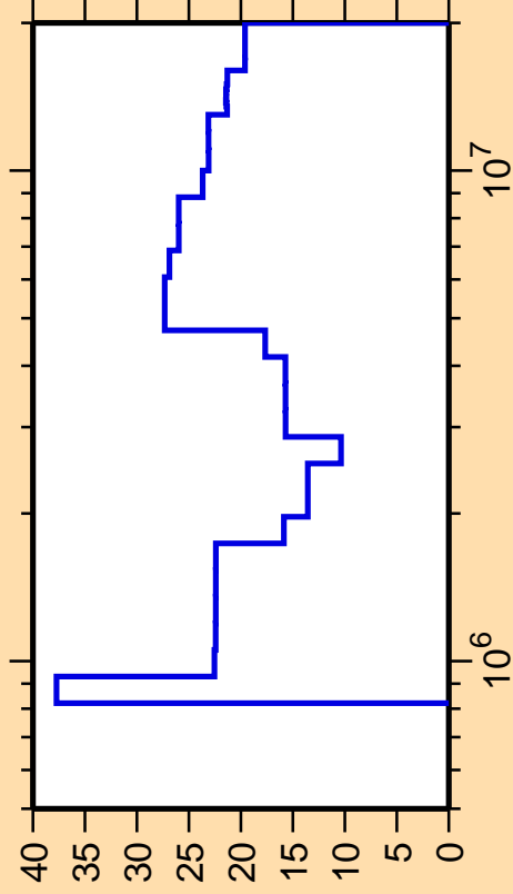
\Delta\sigma/\sigma vs. E for ^{101}\text{Cd}(n,n_2)
