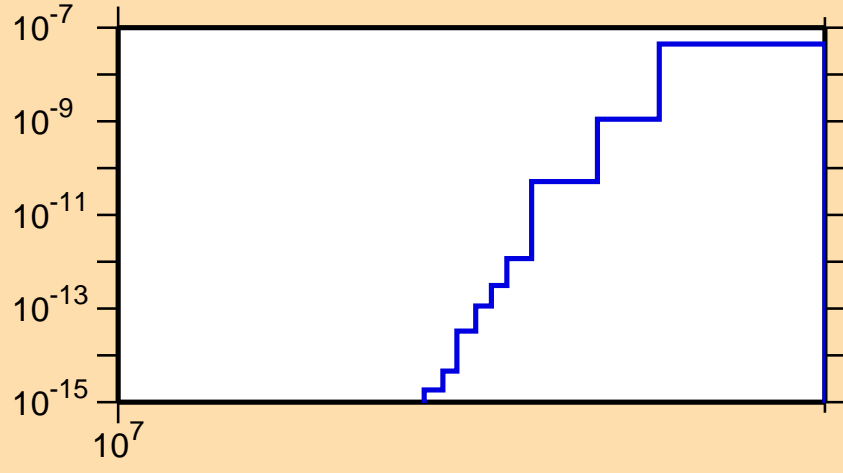
\sigma vs. E for ^{101}\text{Cd}(\text{mt } 34)
