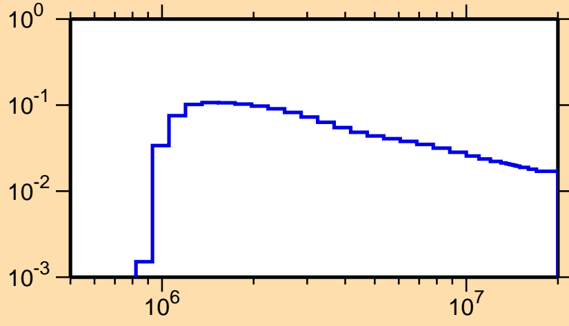
\sigma vs. E for ^{101}\text{Cd}(n,n_2)
