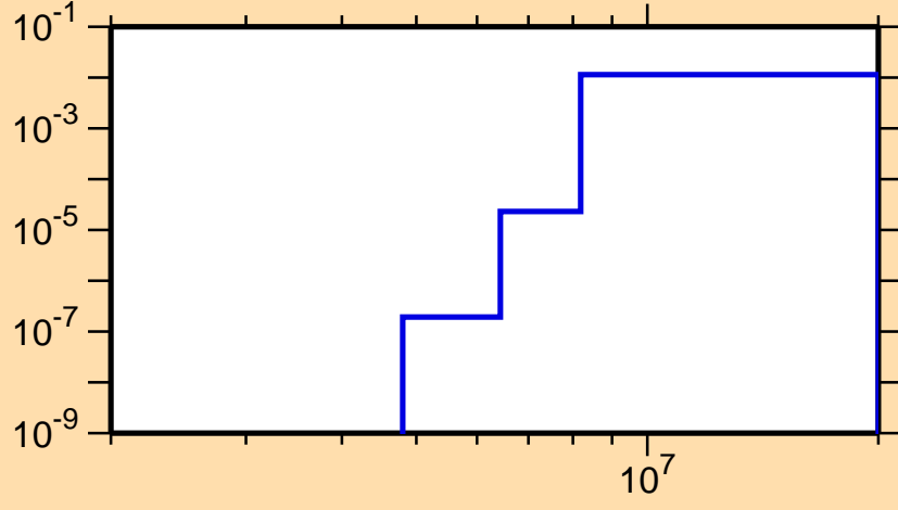
\sigma vs. E for ^{101}\text{Cd}(n,d)
