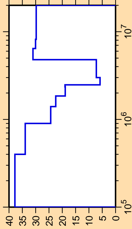
\Delta\sigma/\sigma vs. E for ^{101}\text{Cd}(n,\text{inel.})
