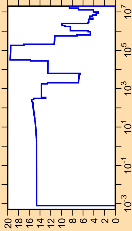
\Delta\sigma/\sigma vs. E for ^{102}\text{Cd}(n,\text{el.})
