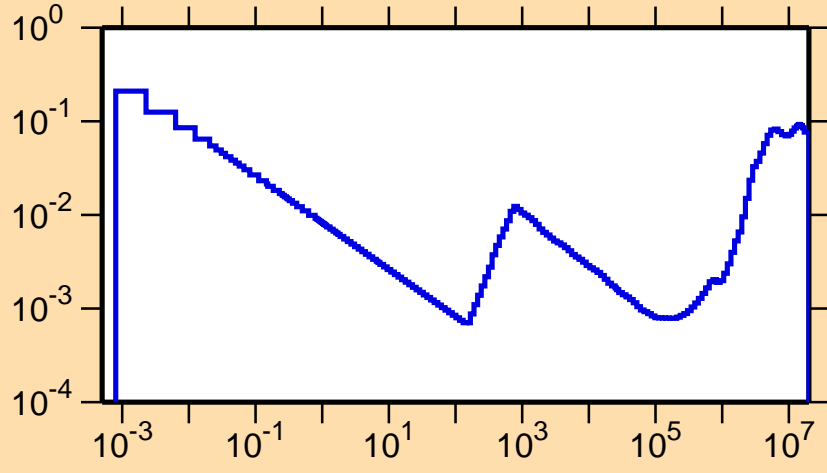
\sigma vs. E for ^{102}\text{Cd}(n,\alpha)
