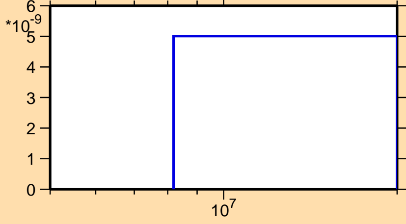
\sigma vs. E for ^{102}\text{Cd}(n,2np)
