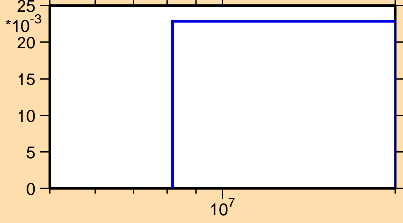
\sigma vs. E for ^{102}\text{Cd}(n,2n)
