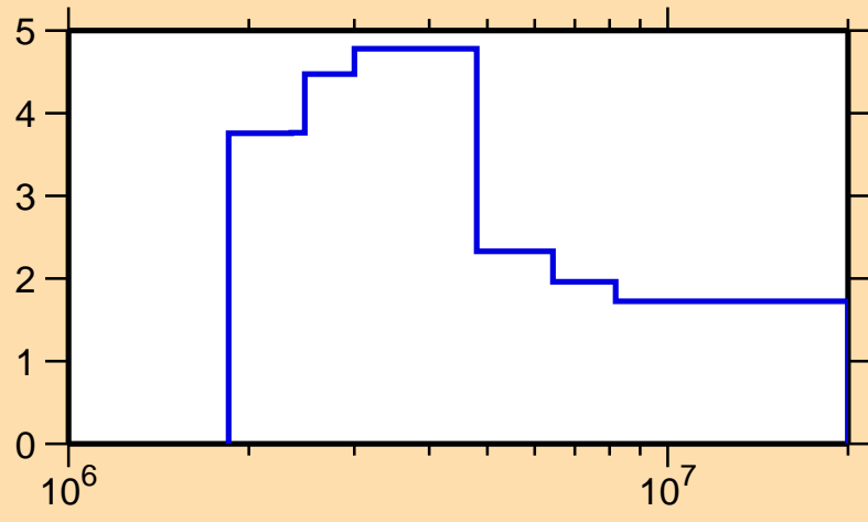
\Delta\sigma/\sigma vs. E for ^{103}\text{Cd}(n,\text{tot.})
