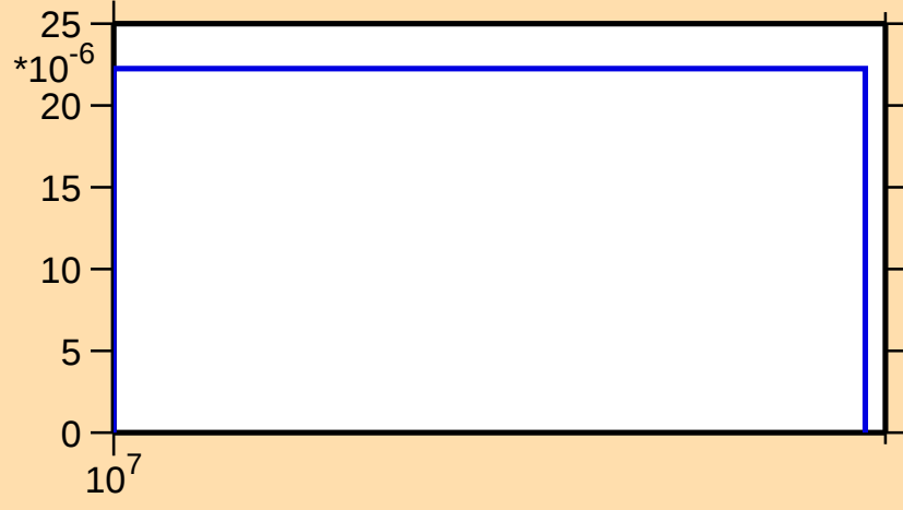
\sigma vs. E for ^{104}\text{Cd}(n,t)
