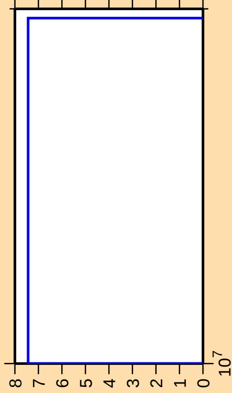
\Delta\sigma/\sigma vs. E for ^{104}\text{Cd}(n,\text{pt})
