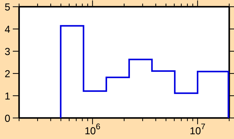
\Delta\sigma/\sigma vs. E for ^{104}\text{Cd}(n,\text{tot.})
