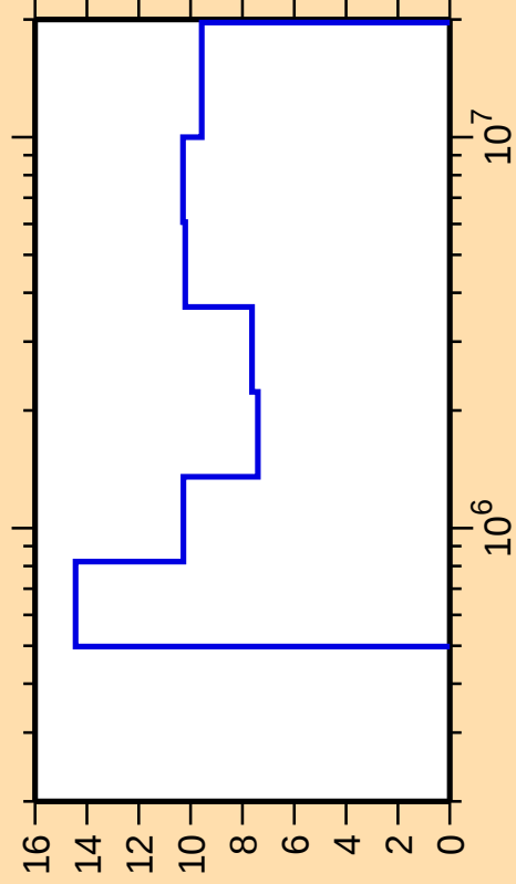
\Delta\sigma/\sigma vs. E for ^{104}\text{Cd}(n,\text{inel.})
