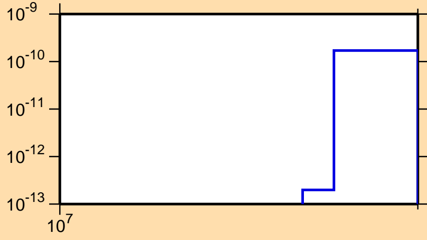
\sigma vs. E for ^{105}\text{Cd}(\text{mt } 34)
