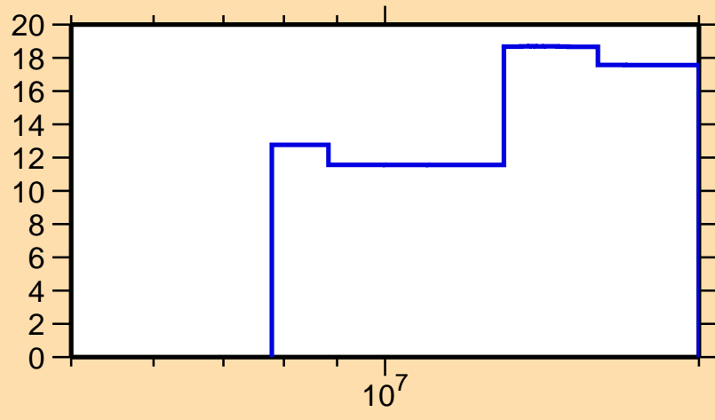
\Delta\sigma/\sigma vs. E for ^{105}\text{Cd}(n,2n)
