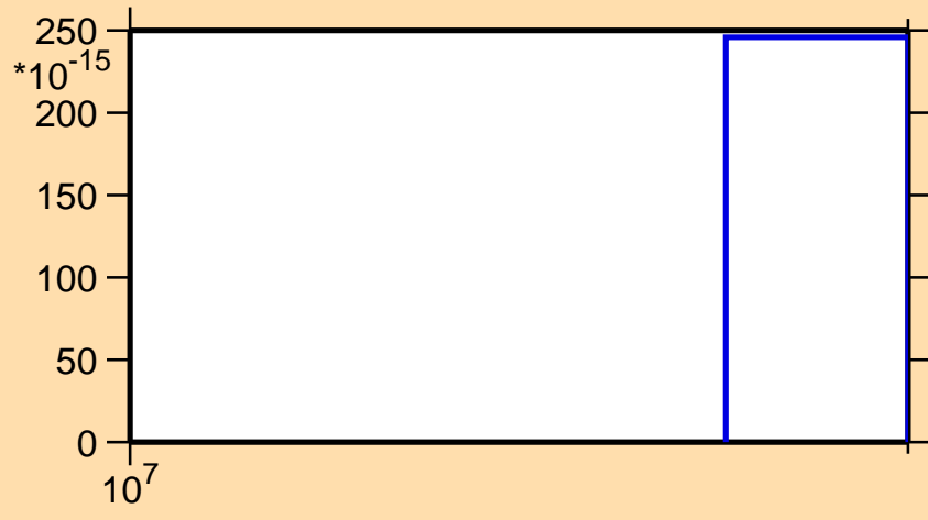
\sigma vs. E for ^{105}\text{Cd}(n,nt)
