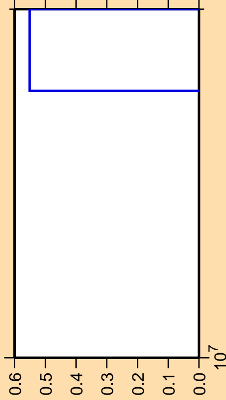
\Delta\sigma/\sigma vs. E for ^{105}\text{Cd}(n,nt)
