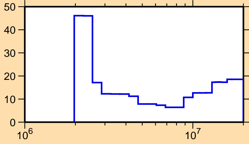
\Delta\sigma/\sigma vs. E for ^{105}\text{Cd}(n,n\text{cont.})
