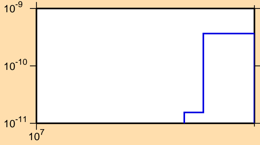
\sigma vs. E for ^{105}\text{Cd}(\text{mt117})
