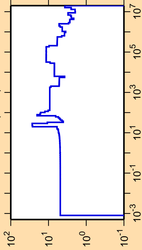
\Delta\sigma/\sigma vs. E for ^{105}\text{Cd}(n,\text{el.})
