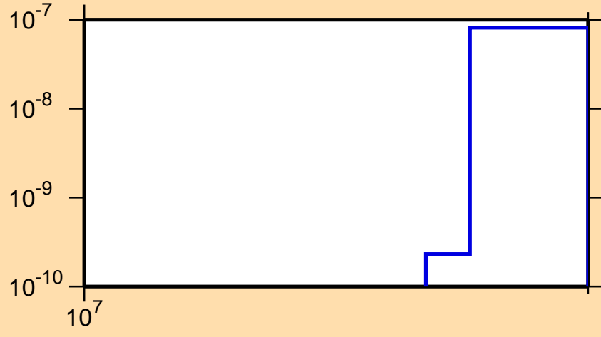
\sigma vs. E for ^{105}\text{Cd}(n,\text{pt})
