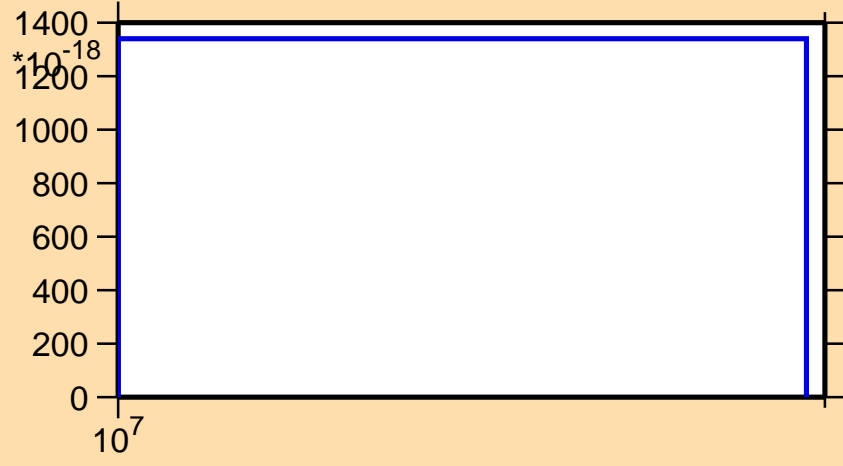
\sigma vs. E for ^{105}\text{Cd}(n,nt)
