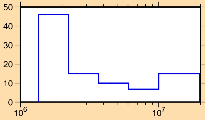
\Delta\sigma/\sigma vs. E for ^{105}\text{Cd}(n,n\text{cont.})
