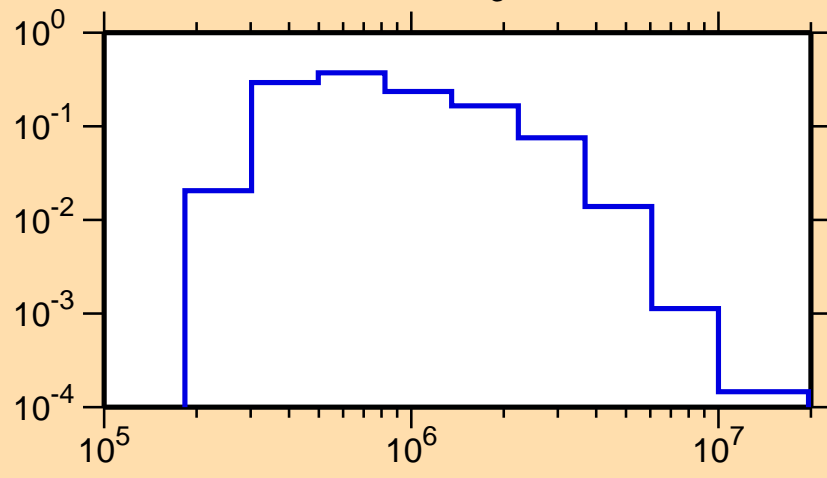
\sigma vs. E for ^{105}\text{Cd}(n,n_3)
