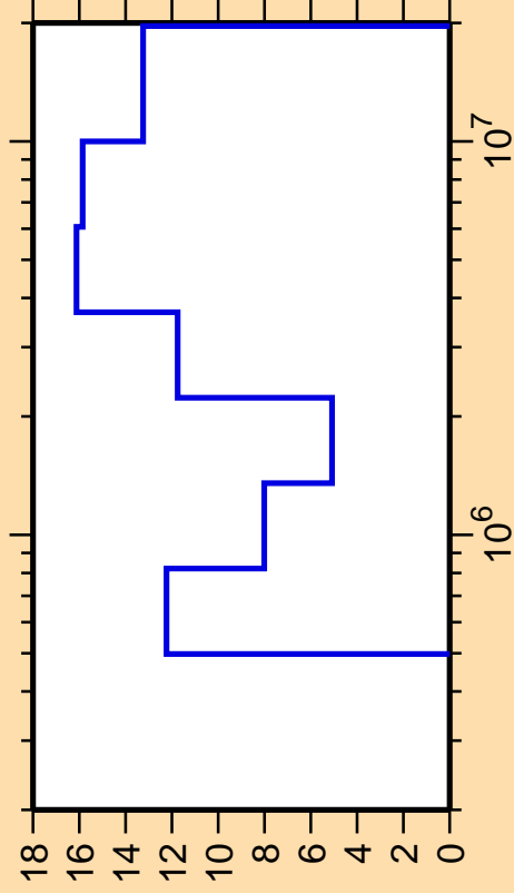
\Delta\sigma/\sigma vs. E for ^{105}\text{Cd}(n,n_4)
