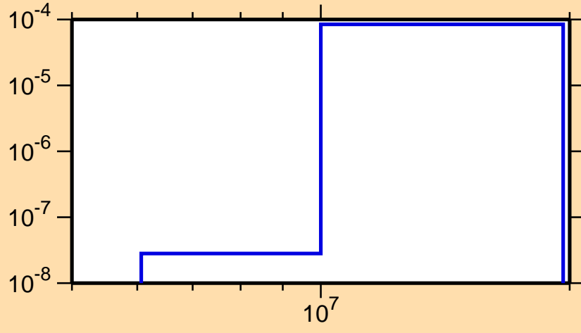
\sigma vs. E for ^{105}\text{Cd}(n,p\alpha)
