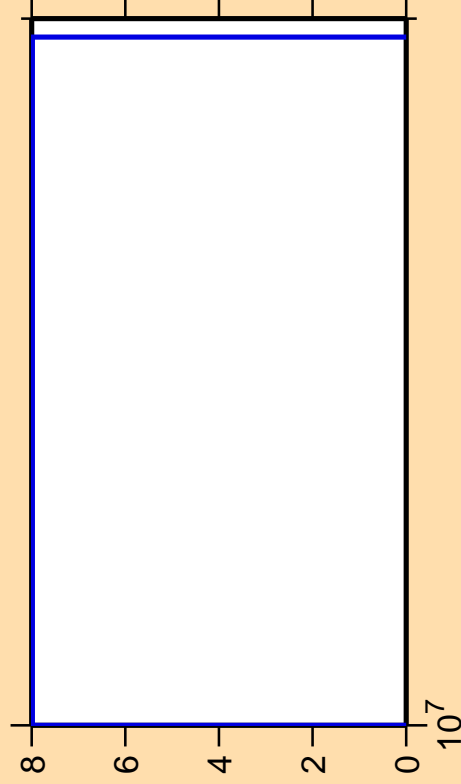
\Delta\sigma/\sigma vs. E for ^{105}\text{Cd}(\text{mt } 45)
