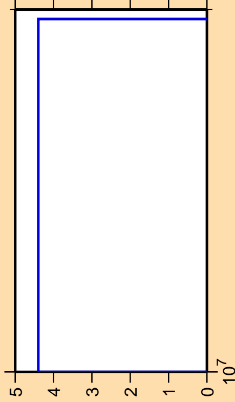
\Delta\sigma/\sigma vs. E for ^{105}\text{Cd}(\text{mt } 34)
