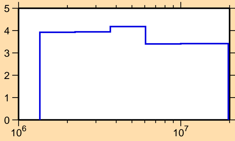
\Delta\sigma/\sigma vs. E for ^{105}\text{Cd}(n,n\text{onel.})
