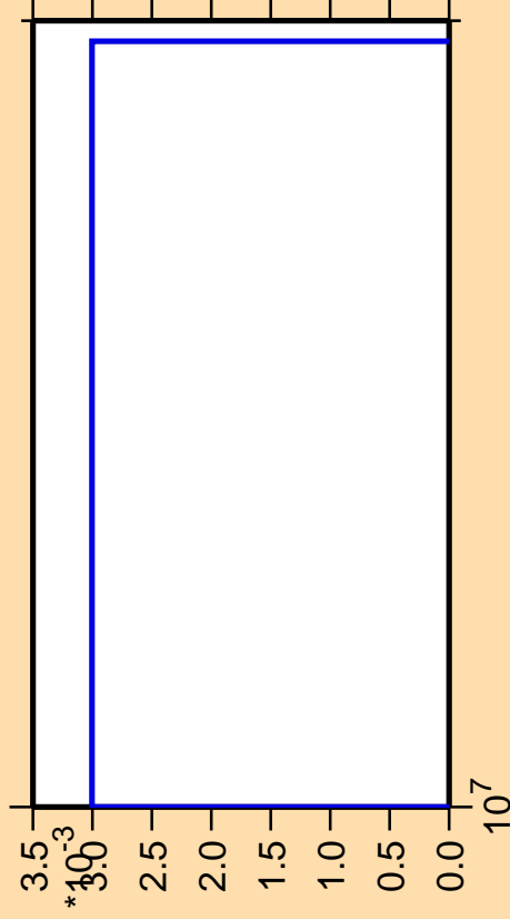
\Delta\sigma/\sigma vs. E for ^{105}\text{Cd}(n,nt)
