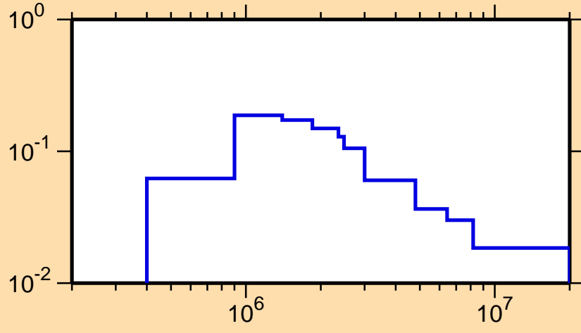
\sigma vs. E for ^{105}\text{Cd}(n,n_4)
