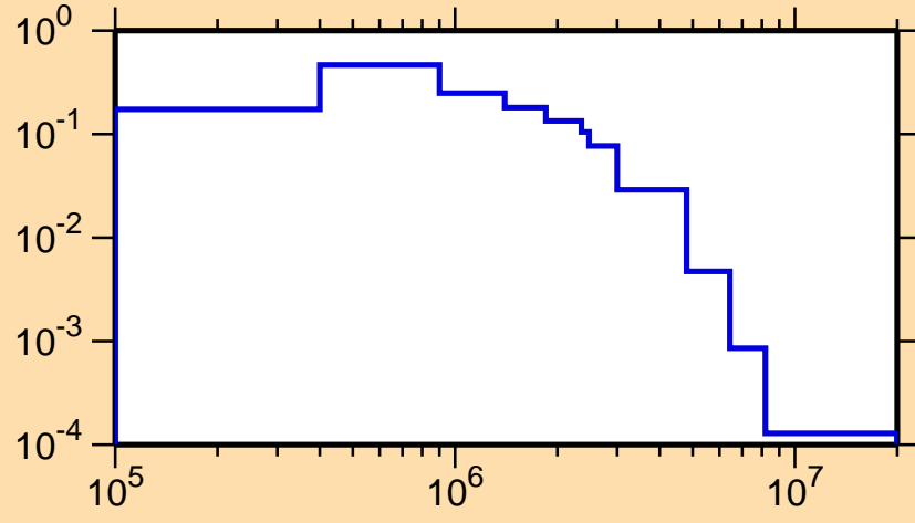
\sigma vs. E for ^{105}\text{Cd}(n,n_2)
