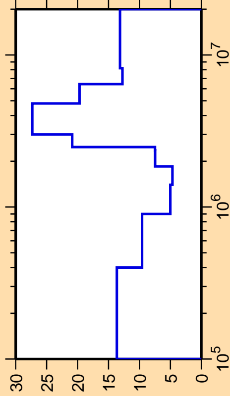
\Delta\sigma/\sigma vs. E for ^{105}\text{Cd}(n,n_2)
