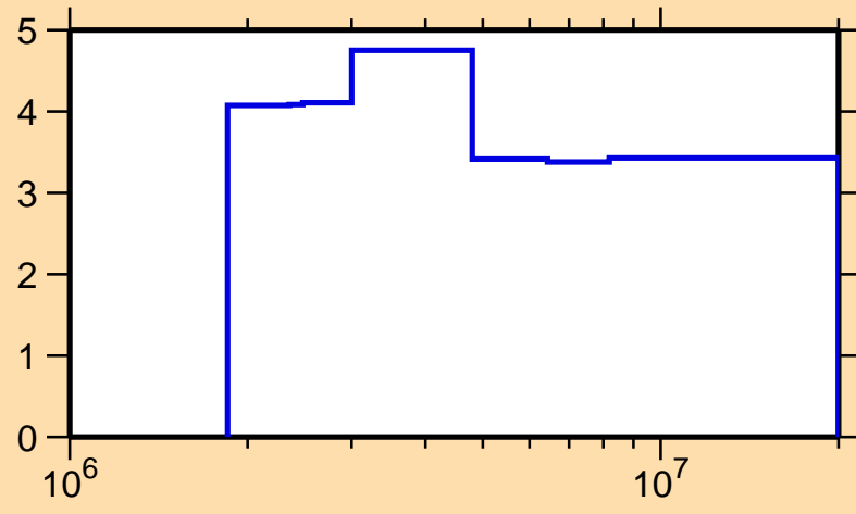
\Delta\sigma/\sigma vs. E for ^{105}\text{Cd}(n,\text{nonel.})
