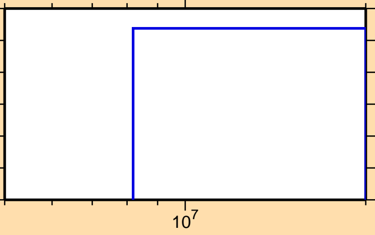
\sigma vs. E for ^{105}\text{Cd}(\text{mt } 45)
