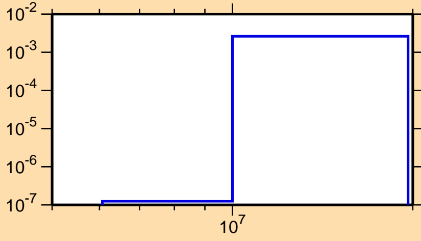
\sigma vs. E for ^{106}\text{Cd}(n,d)
