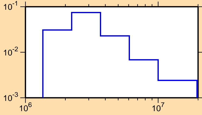
\sigma vs. E for ^{106}\text{Cd}(n,n_4)
