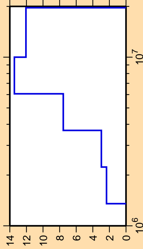
\Delta\sigma/\sigma vs. E for ^{106}\text{Cd}(n,n_4)
