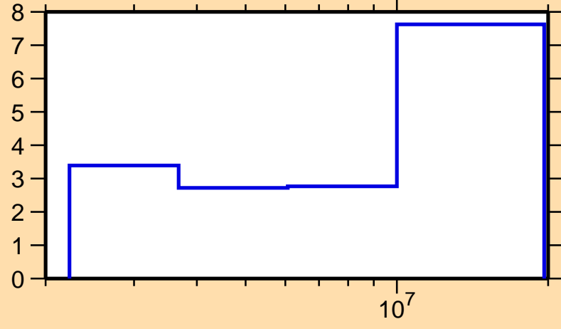
\Delta\sigma/\sigma vs. E for ^{106}\text{Cd}(n,n\text{cont.})
