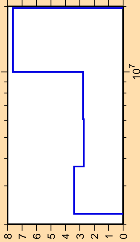
\Delta\sigma/\sigma vs. E for ^{106}\text{Cd}(n,n\text{cont.})
