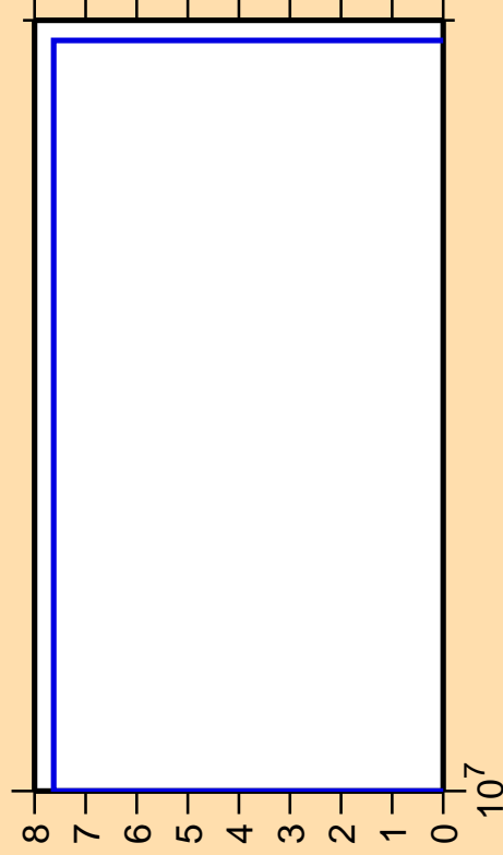
\Delta\sigma/\sigma vs. E for ^{106}\text{Cd}(n,n\text{cont.})
