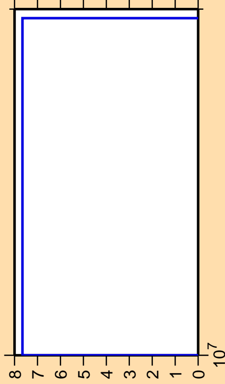
\Delta\sigma/\sigma vs. E for ^{106}\text{Cd}(n,n_1)
