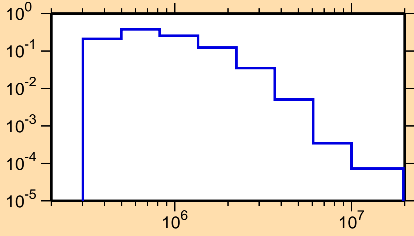
\sigma vs. E for ^{107}\text{Cd}(n,n_2)
