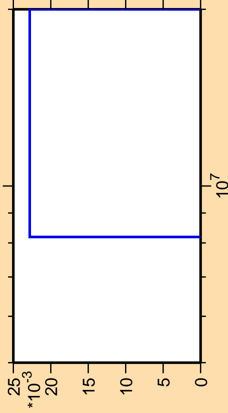
\Delta\sigma/\sigma vs. E for ^{107}\text{Cd}(n,nt)
