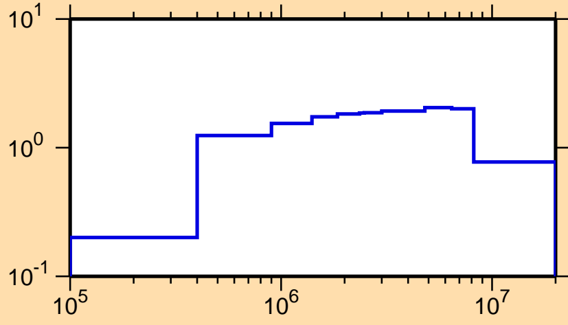
\sigma vs. E for ^{107}\text{Cd}(n,\text{inel.})
