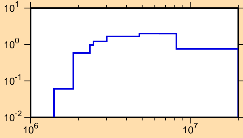
\sigma vs. E for ^{107}\text{Cd}(n,n\text{cont.})
