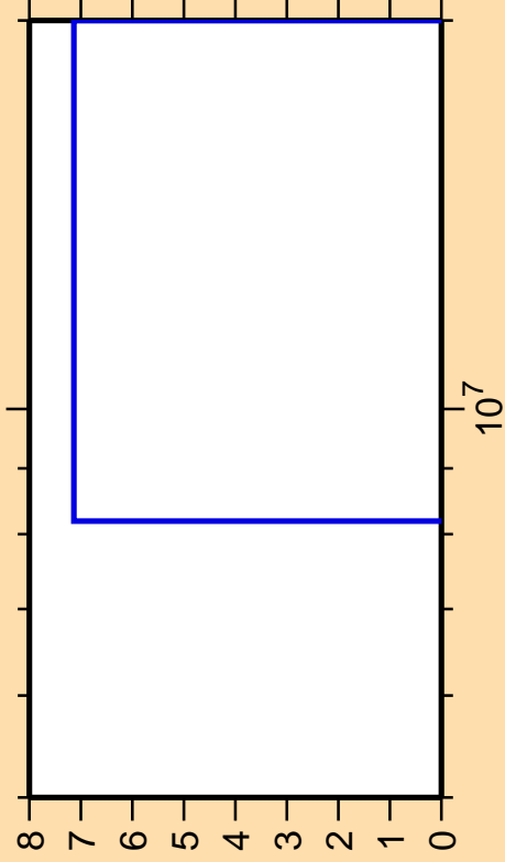
\Delta\sigma/\sigma vs. E for ^{107}\text{Cd}(n,\text{pd})
