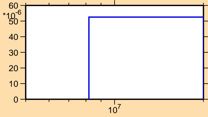
\sigma vs. E for ^{107}\text{Cd}(n,t)
