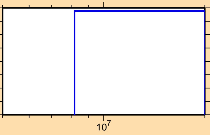
\sigma vs. E for ^{107}\text{Cd}(n,3n)
