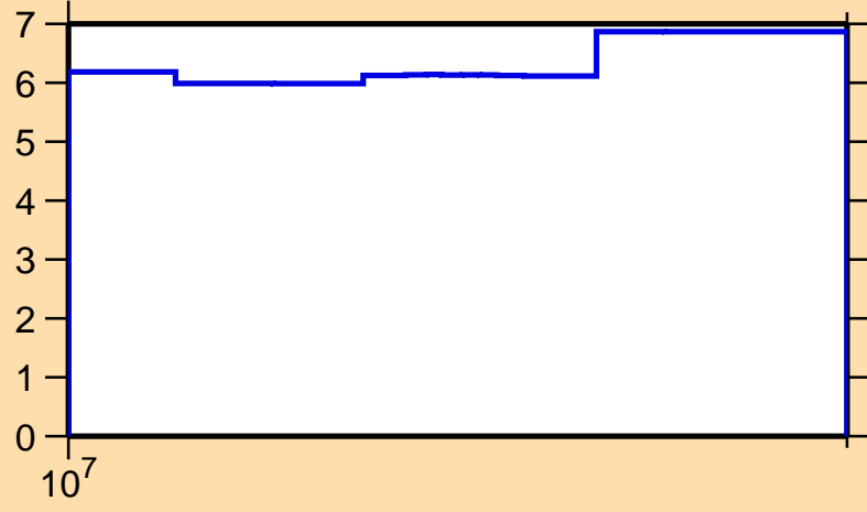
\Delta\sigma/\sigma vs. E for ^{108}\text{Cd}(n,2n)
