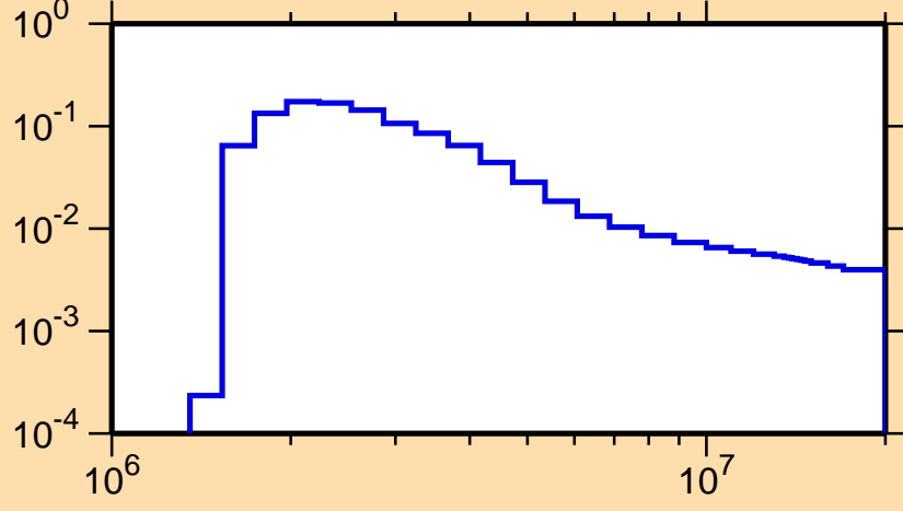
\sigma vs. E for ^{108}\text{Cd}(n,n_2)
