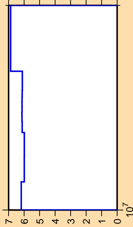
\Delta\sigma/\sigma vs. E for ^{108}\text{Cd}(n,2n)
