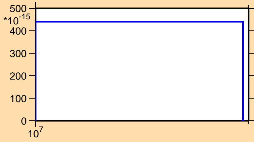
\sigma vs. E for ^{108}\text{Cd}(n,2np)
