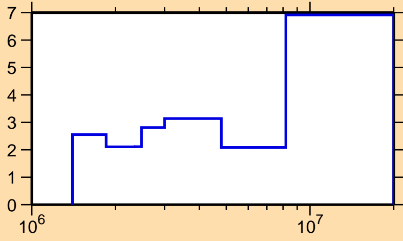
\Delta\sigma/\sigma vs. E for ^{108}\text{Cd}(n,\text{inel.})
