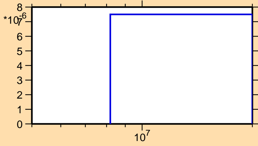
\sigma vs. E for ^{108}\text{Cd}(n,t)
