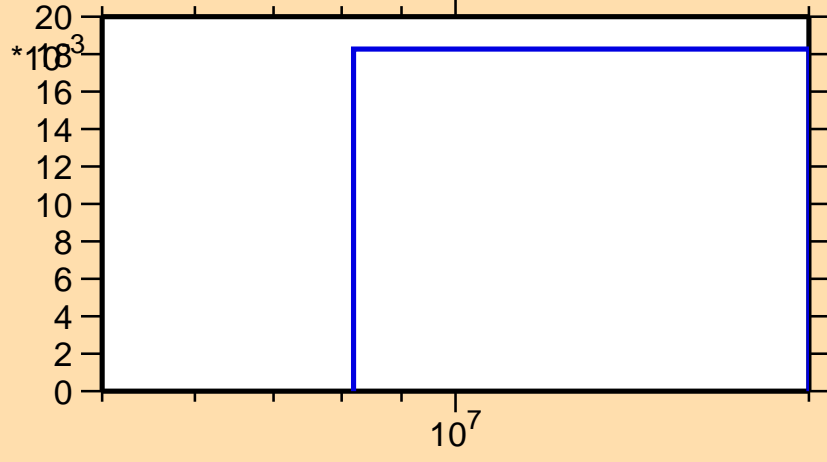
\sigma vs. E for ^{108}\text{Cd}(n,np)
