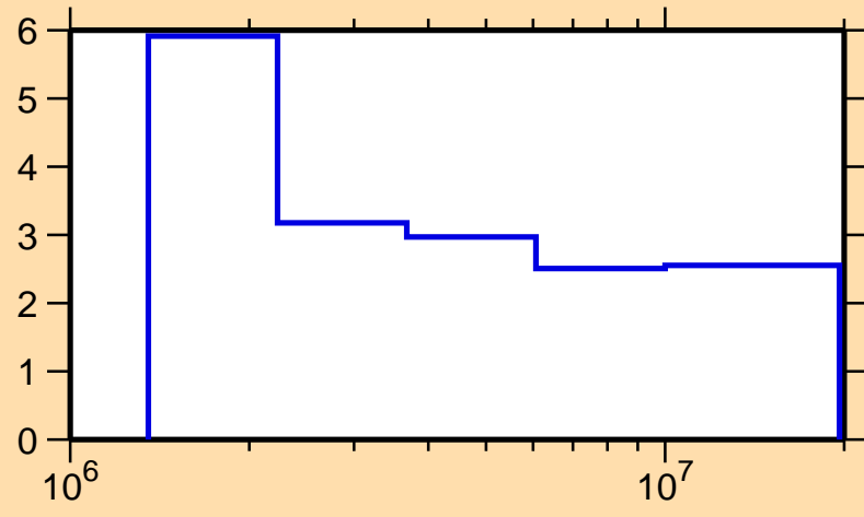
\Delta\sigma/\sigma vs. E for ^{109}\text{Cd}(n,n\text{onel.})
