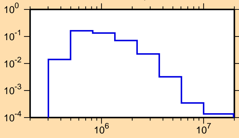
\sigma vs. E for ^{109}\text{Cd}(n,n_4)
