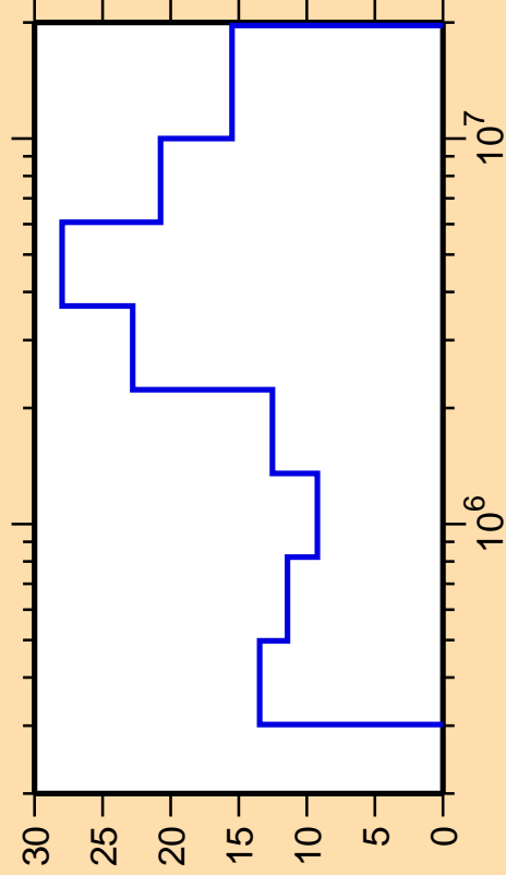
\Delta\sigma/\sigma vs. E for ^{109}\text{Cd}(n,n_4)
