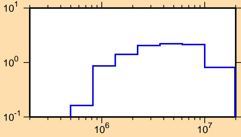
\sigma vs. E for ^{110}\text{Cd}(n,\text{inel.})
