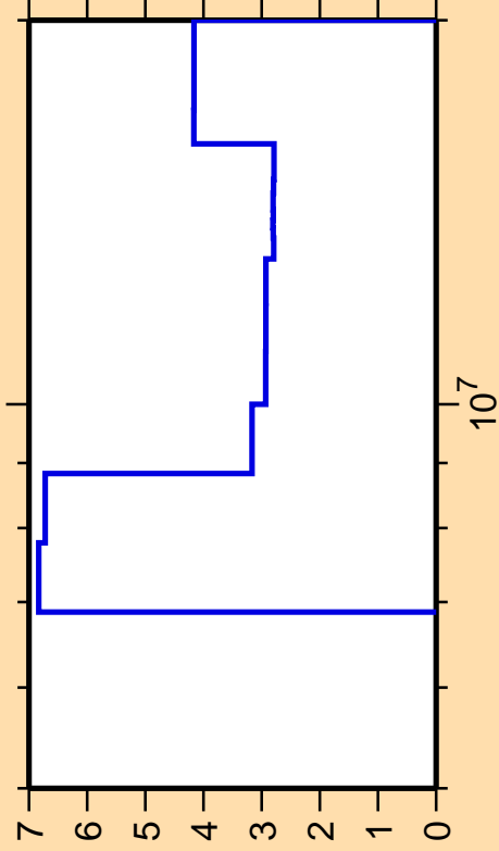
\Delta\sigma/\sigma vs. E for ^{111}\text{Cd}(n,2n)
