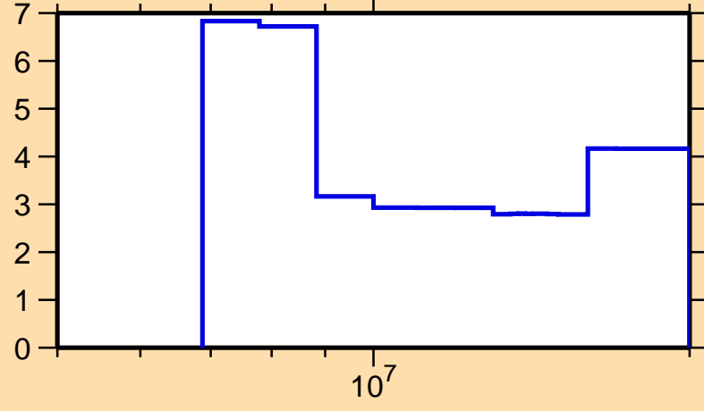
\Delta\sigma/\sigma vs. E for ^{111}\text{Cd}(n,2n)
