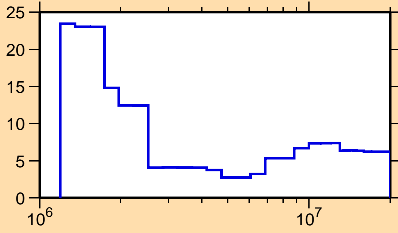
\Delta\sigma/\sigma vs. E for ^{111}\text{Cd}(n,n\text{cont.})
