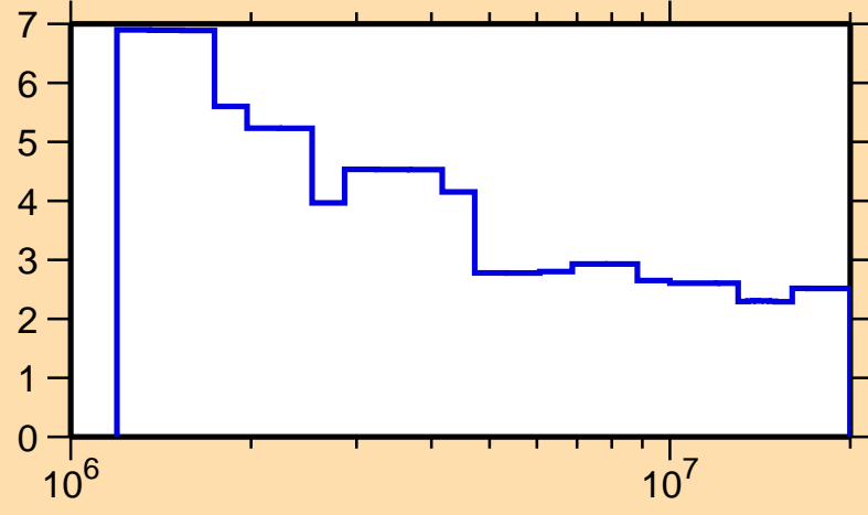
\Delta\sigma/\sigma vs. E for ^{111}\text{Cd}(n,n\text{onel.})
