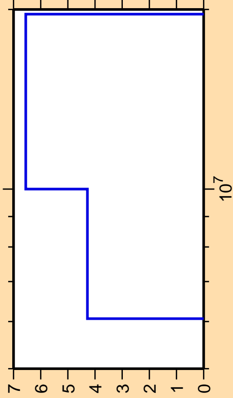
\Delta\sigma/\sigma vs. E for ^{111}\text{Cd}(n,n\text{cont.})
