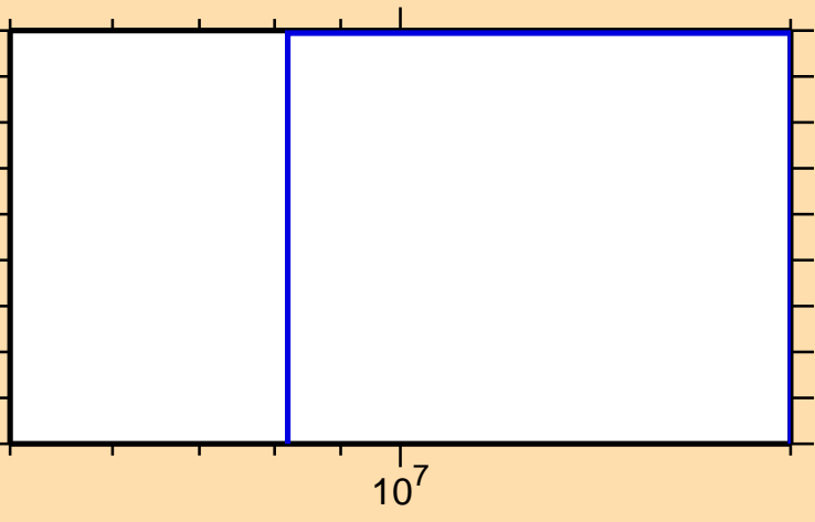
\sigma vs. E for ^{111}\text{Cd}(n,\text{nd})
