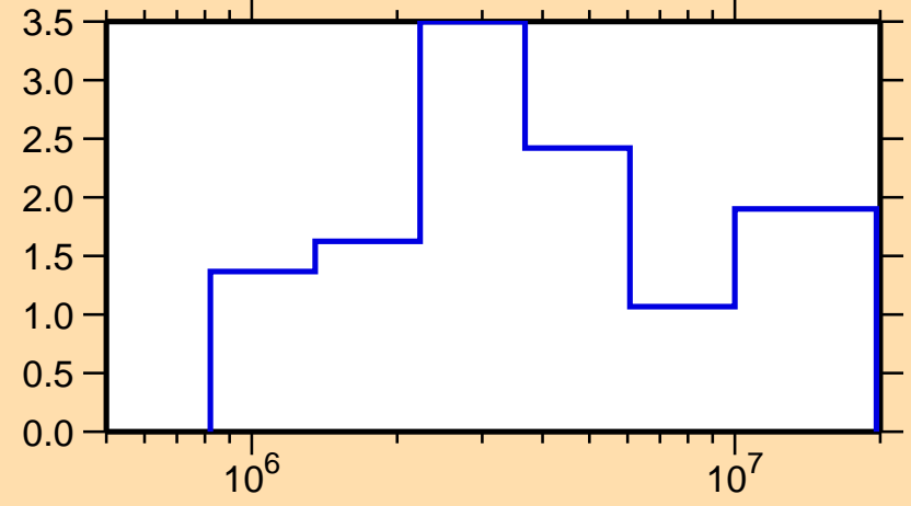
\Delta\sigma/\sigma vs. E for ^{111}\text{Cd}(n,\text{tot.})
