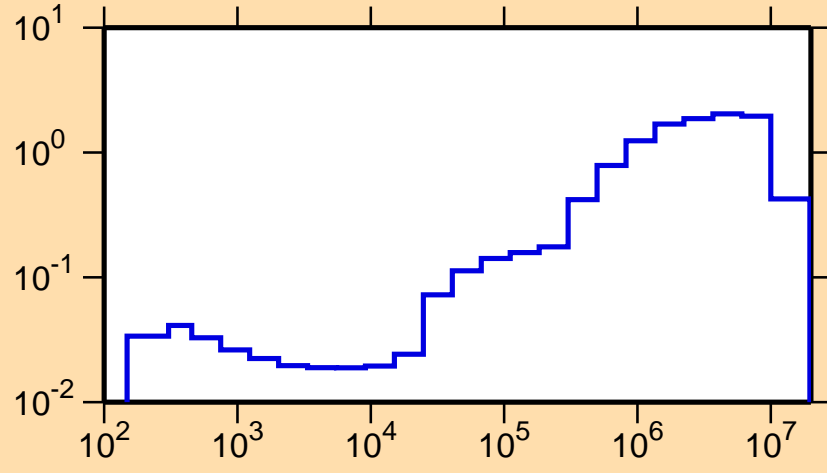
\sigma vs. E for ^{111}\text{Cd}(n,\text{inel.})
