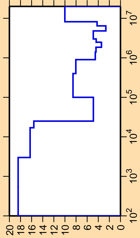
\Delta\sigma/\sigma vs. E for ^{111}\text{Cd}(n,\text{inel.})
