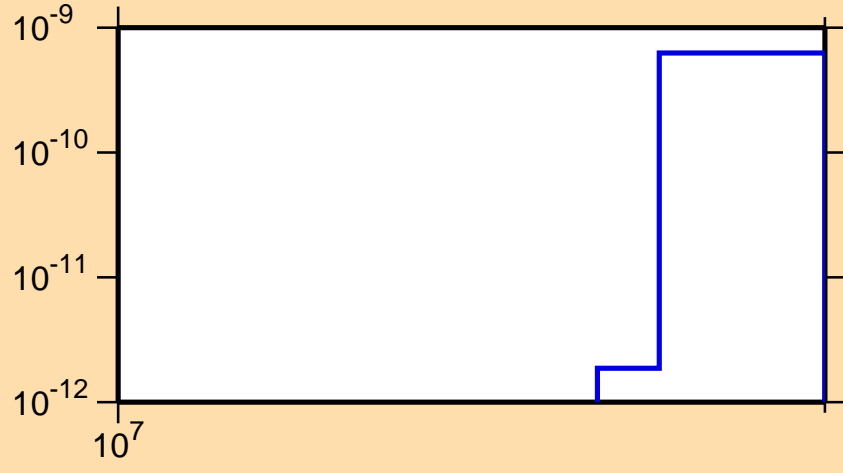
\sigma vs. E for ^{112}\text{Cd}(n,\text{He3})
