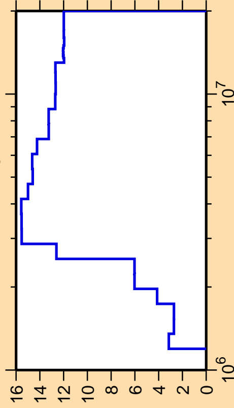
\Delta\sigma/\sigma vs. E for ^{112}\text{Cd}(n,n_3)
