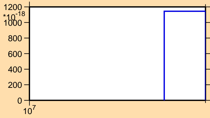
\sigma vs. E for ^{112}\text{Cd}(n,2np)
