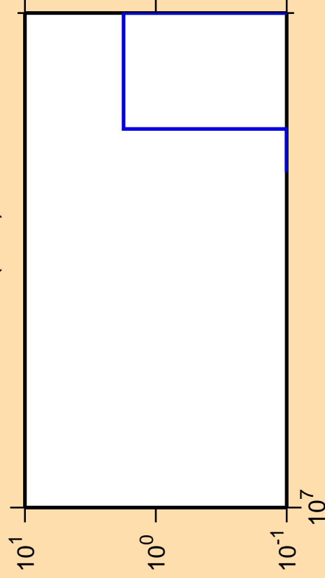
\Delta\sigma/\sigma vs. E for ^{112}\text{Cd}(n,nt)
