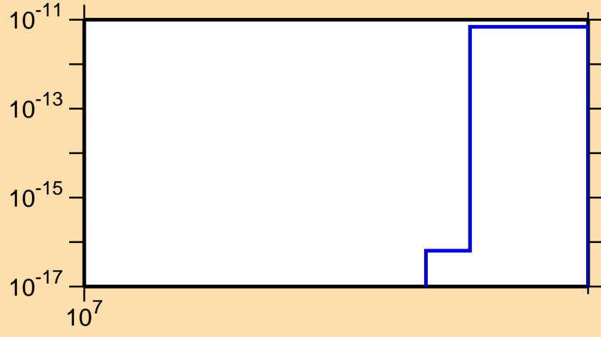
\sigma vs. E for ^{112}\text{Cd}(n,2n\alpha)
