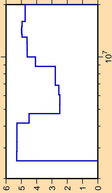
\Delta\sigma/\sigma vs. E for ^{112}\text{Cd}(n,n\text{cont.})
