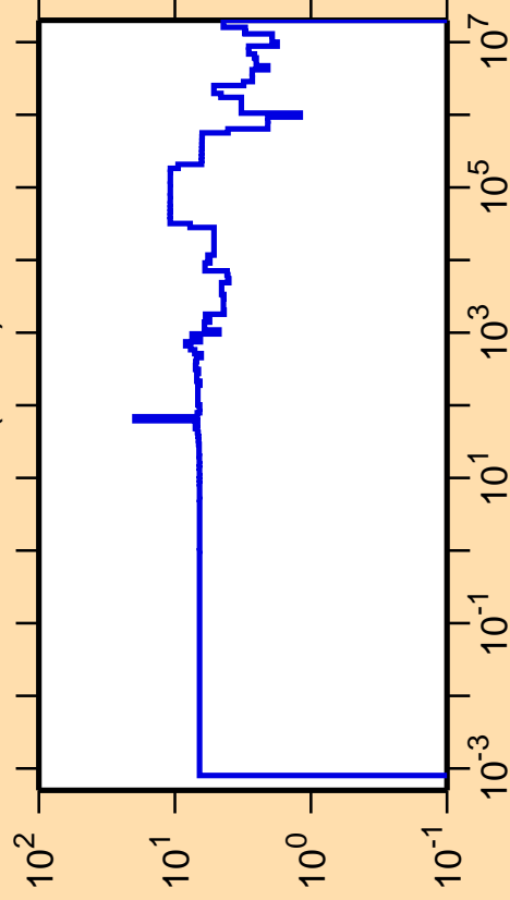
\Delta\sigma/\sigma vs. E for ^{112}\text{Cd}(n,\text{el.})
