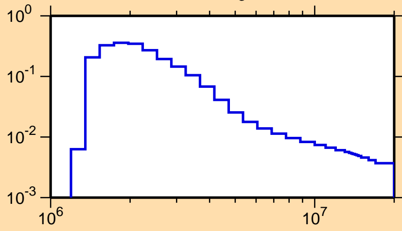
\sigma vs. E for ^{112}\text{Cd}(n,n_3)
