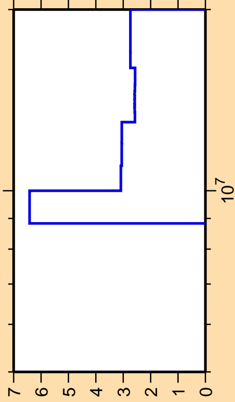
\Delta\sigma/\sigma vs. E for ^{112}\text{Cd}(n,2n)
