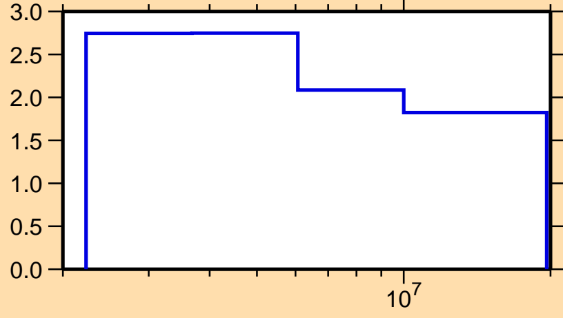
\Delta\sigma/\sigma vs. E for ^{112}\text{Cd}(n,n\text{onel.})
