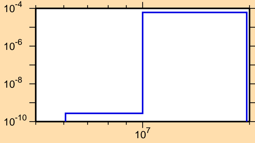
\sigma vs. E for ^{112}\text{Cd}(n,n\alpha)
