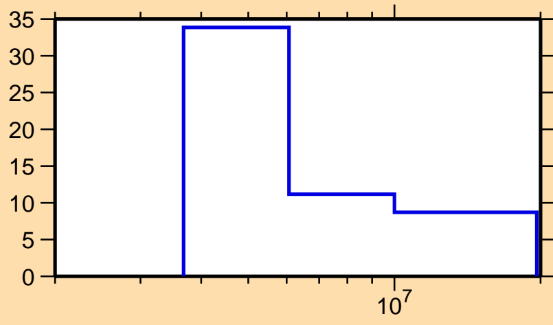
\Delta\sigma/\sigma vs. E for ^{112}\text{Cd}(n,p)
