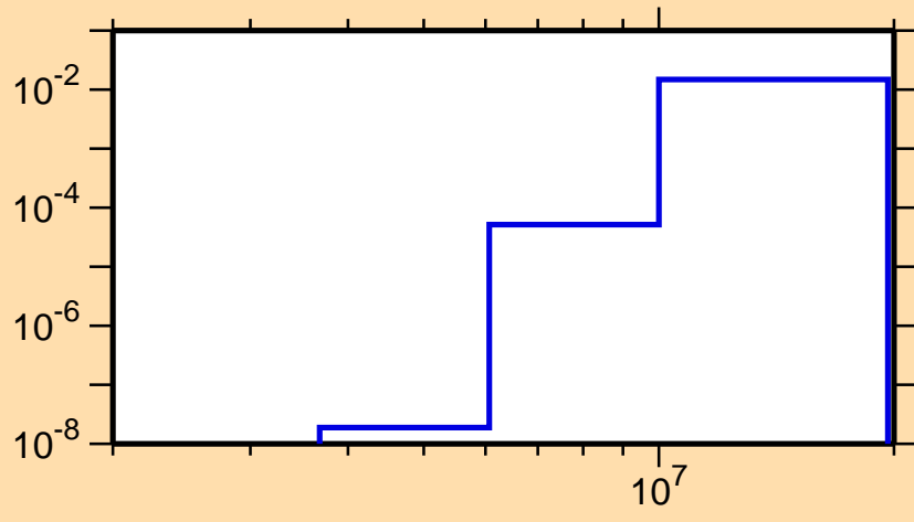
\sigma vs. E for ^{112}\text{Cd}(n,p)
