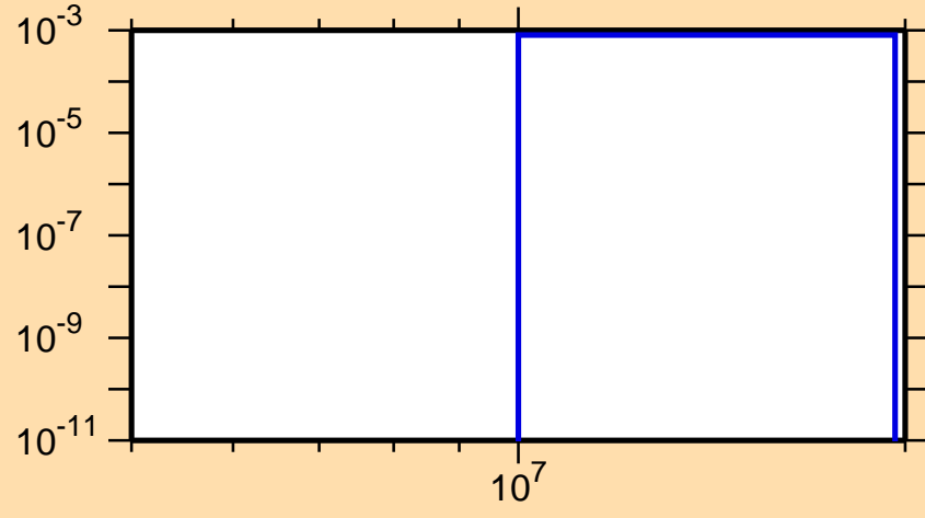
\sigma vs. E for ^{112}\text{Cd}(n,d)
