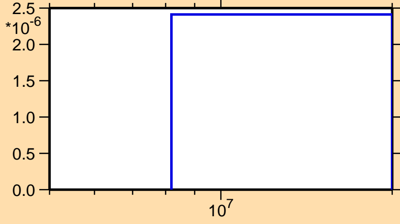
\sigma vs. E for ^{112}\text{Cd}(n,t)
