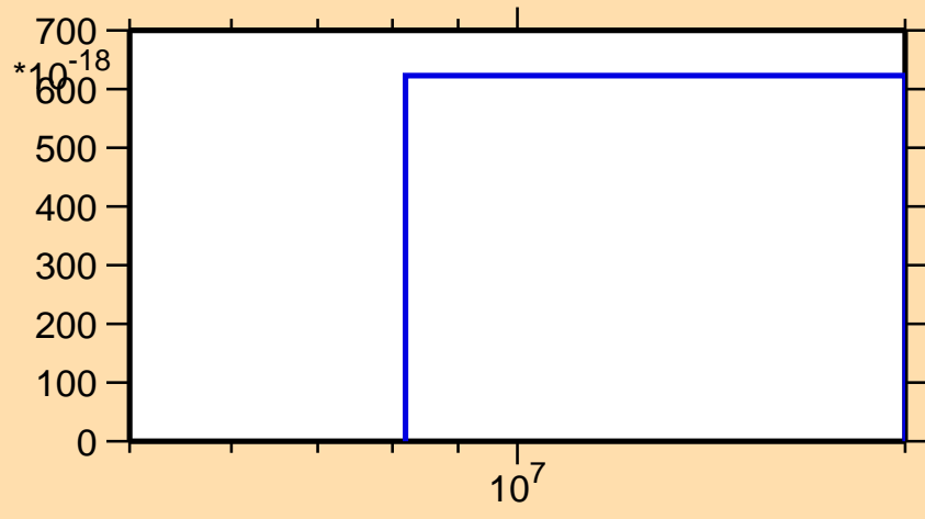
\sigma vs. E for ^{112}\text{Cd}(n,p\alpha)
