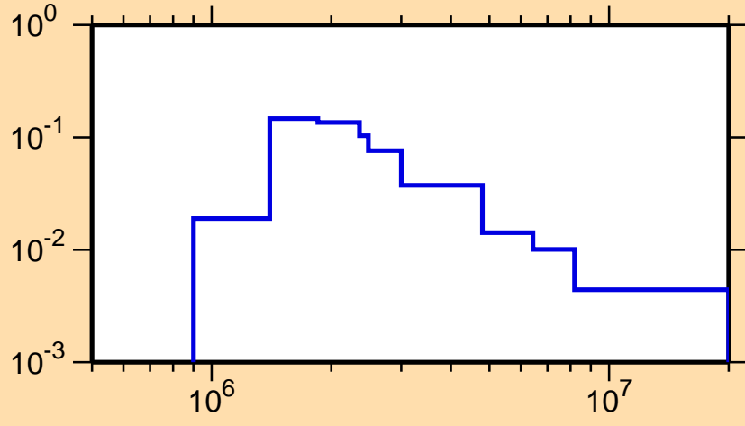
\sigma vs. E for ^{112}\text{Cd}(n,n_2)
