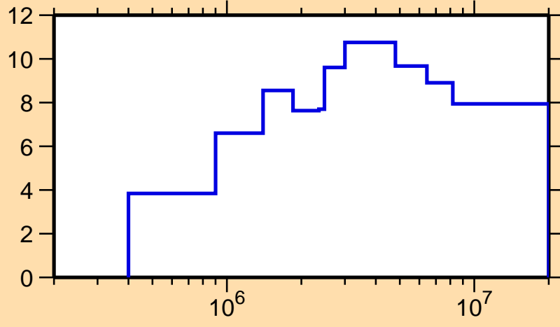
\Delta\sigma/\sigma vs. E for ^{112}\text{Cd}(n,n_1)
