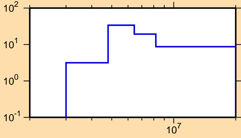
\Delta\sigma/\sigma vs. E for ^{112}\text{Cd}(n,p)
