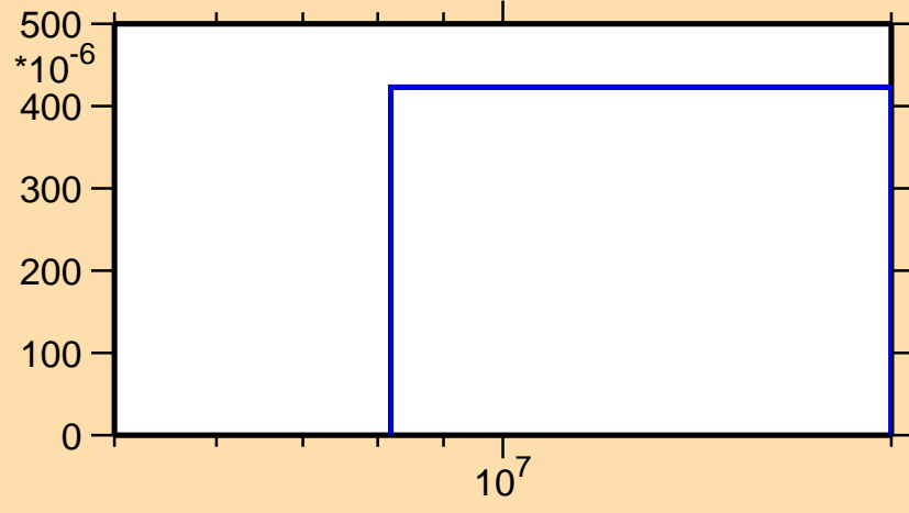
\sigma vs. E for ^{112}\text{Cd}(n,np)
