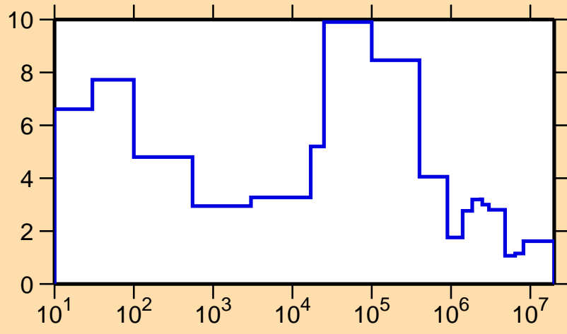
\Delta\sigma/\sigma vs. E for ^{112}\text{Cd}(n,\text{tot.})
