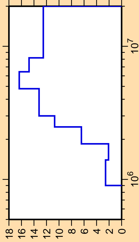
\Delta\sigma/\sigma vs. E for ^{112}\text{Cd}(n,n_2)
