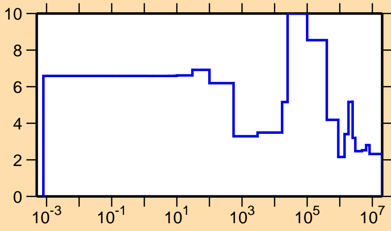
\Delta\sigma/\sigma vs. E for ^{112}\text{Cd}(n,\text{el.})
