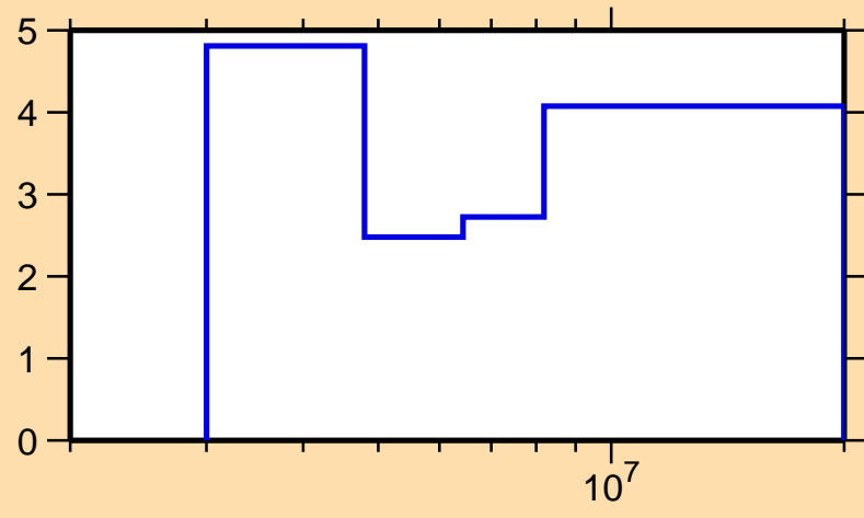
\Delta\sigma/\sigma vs. E for ^{112}\text{Cd}(n,n\text{cont.})
