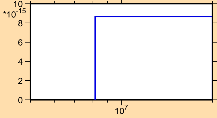
\sigma vs. E for ^{112}\text{Cd}(n,nt)
