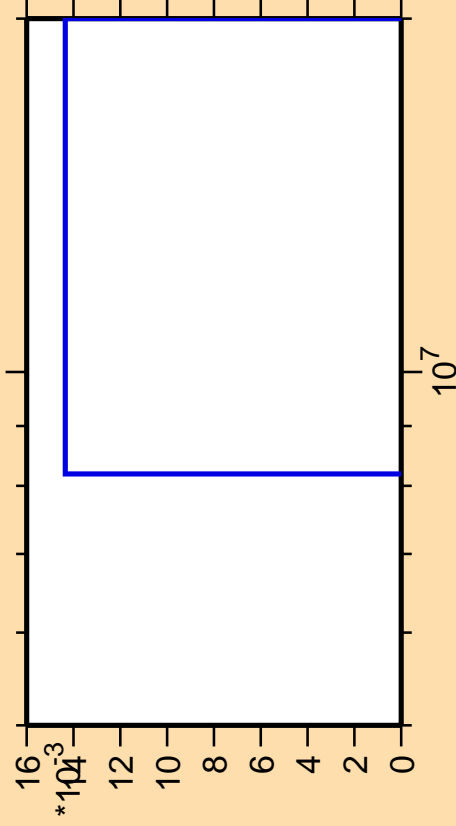
\Delta\sigma/\sigma vs. E for ^{112}\text{Cd}(n,nt)
