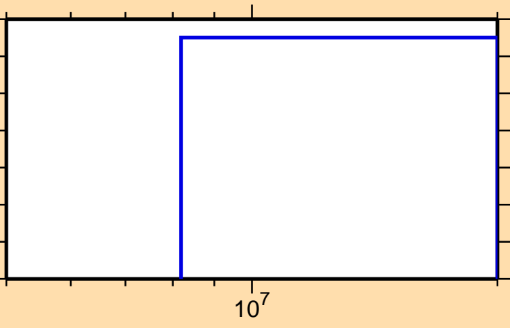
\sigma vs. E for ^{112}\text{Cd}(n,d)
