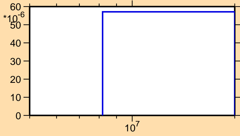
\sigma vs. E for ^{112}\text{Cd}(n,3n)
