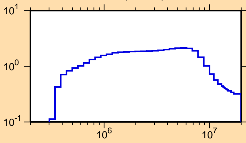
\sigma vs. E for ^{113}\text{Cd}(n,\text{inel.})
