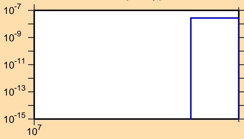
\sigma vs. E for ^{113}\text{Cd}(n,2np)
