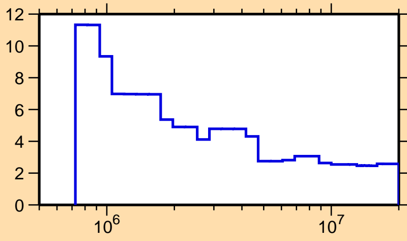
\Delta\sigma/\sigma vs. E for ^{113}\text{Cd}(n,n\text{onel.})
