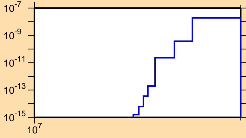
\sigma vs. E for ^{113}\text{Cd}(n,2n\alpha)
