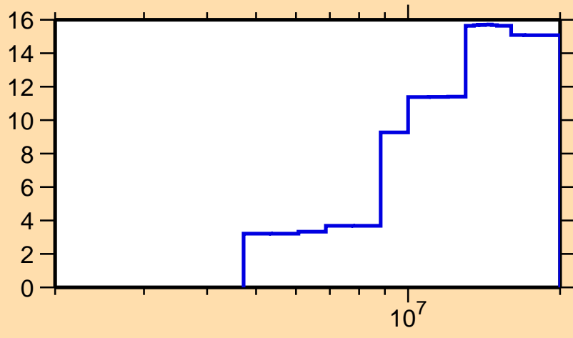
\Delta\sigma/\sigma vs. E for ^{114}\text{Cd}(n,n\text{cont.})
