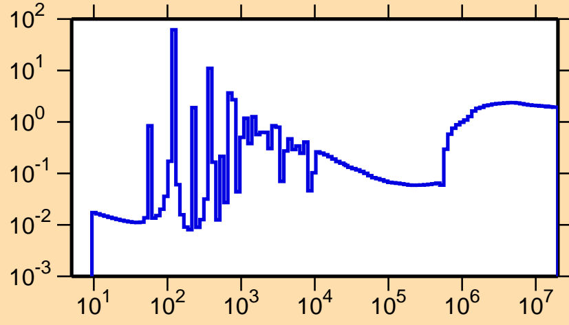
\sigma vs. E for ^{114}\text{Cd}(n,\text{nonel.})
