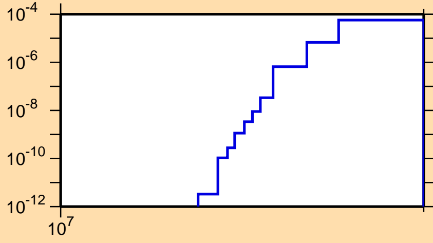
\sigma vs. E for ^{114}\text{Cd}(n,t)
