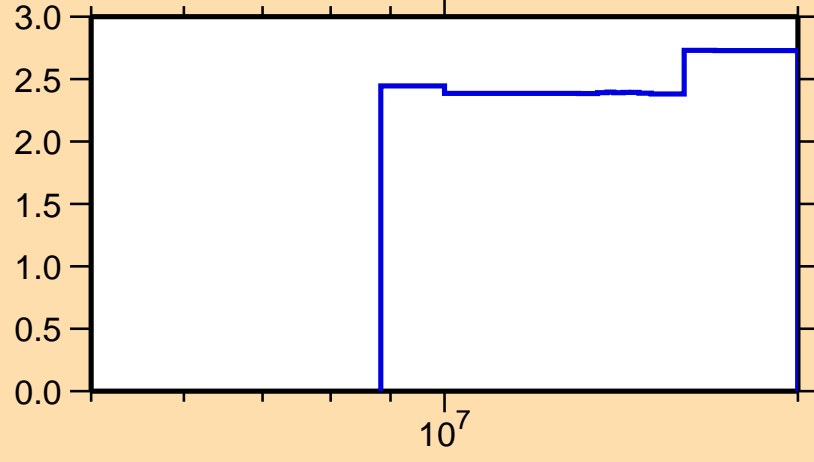
\Delta\sigma/\sigma vs. E for ^{114}\text{Cd}(n,\text{nonel.})
