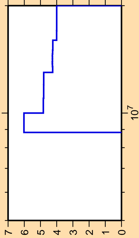
\Delta\sigma/\sigma vs. E for ^{114}\text{Cd}(n,2n)
