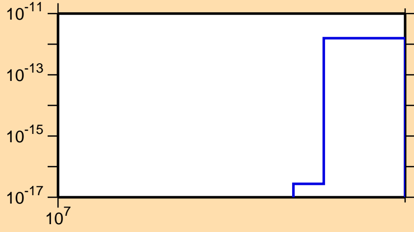
\sigma vs. E for ^{114}\text{Cd}(n,nt)
