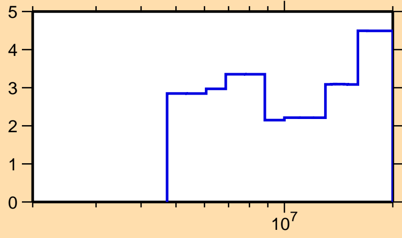
\Delta\sigma/\sigma vs. E for ^{114}\text{Cd}(n,\text{el.})
