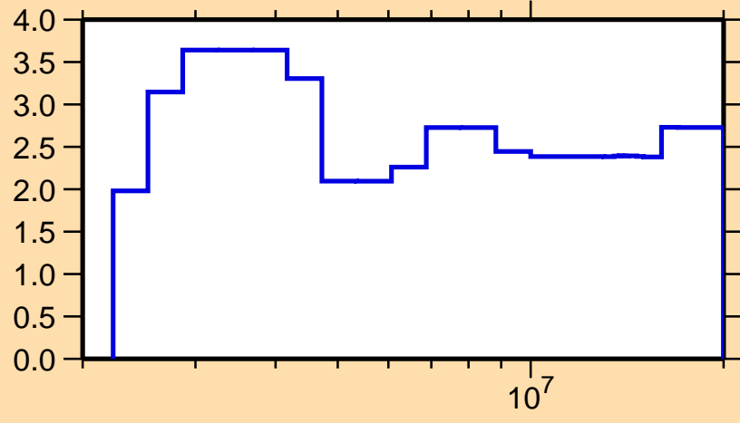
\Delta\sigma/\sigma vs. E for ^{114}\text{Cd}(n,n\text{onel.})
