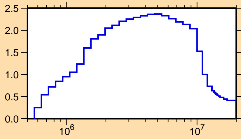
\sigma vs. E for ^{114}\text{Cd}(n,\text{inel.})
