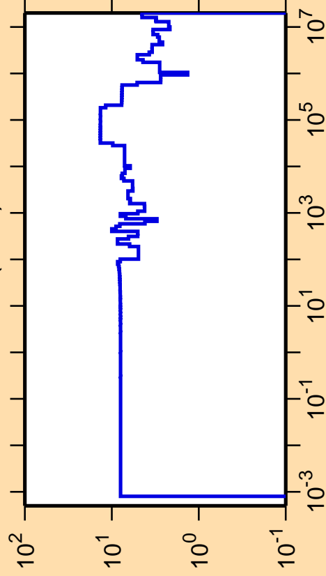
\Delta\sigma/\sigma vs. E for ^{114}\text{Cd}(n,\text{el.})
