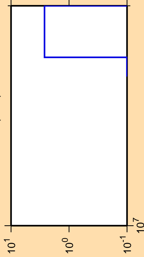
\Delta\sigma/\sigma vs. E for ^{114}\text{Cd}(n,nt)
