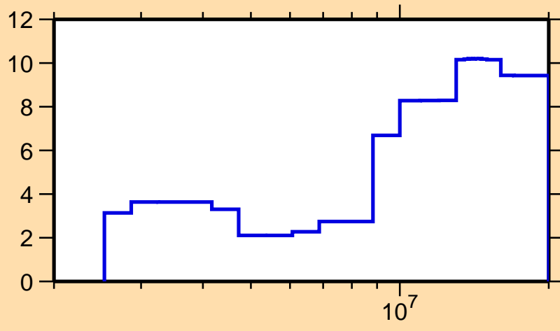
\Delta\sigma/\sigma vs. E for ^{114}\text{Cd}(n,\text{inel.})
