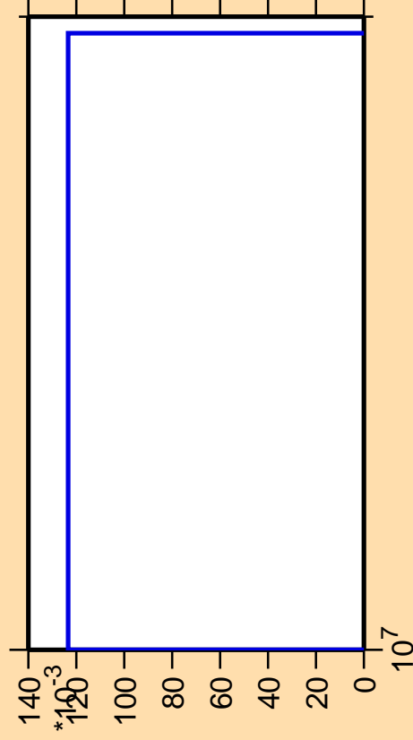
\Delta\sigma/\sigma vs. E for ^{114}\text{Cd}(n,\text{nd})
