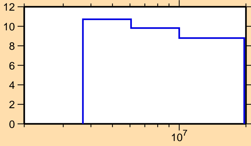
\Delta\sigma/\sigma vs. E for ^{114}\text{Cd}(n,n_1)
