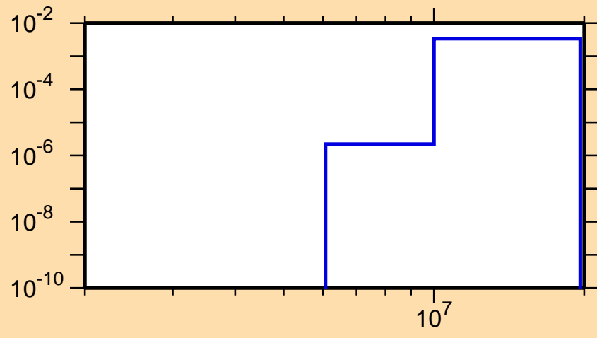
\sigma vs. E for ^{114}\text{Cd}(n,p)
